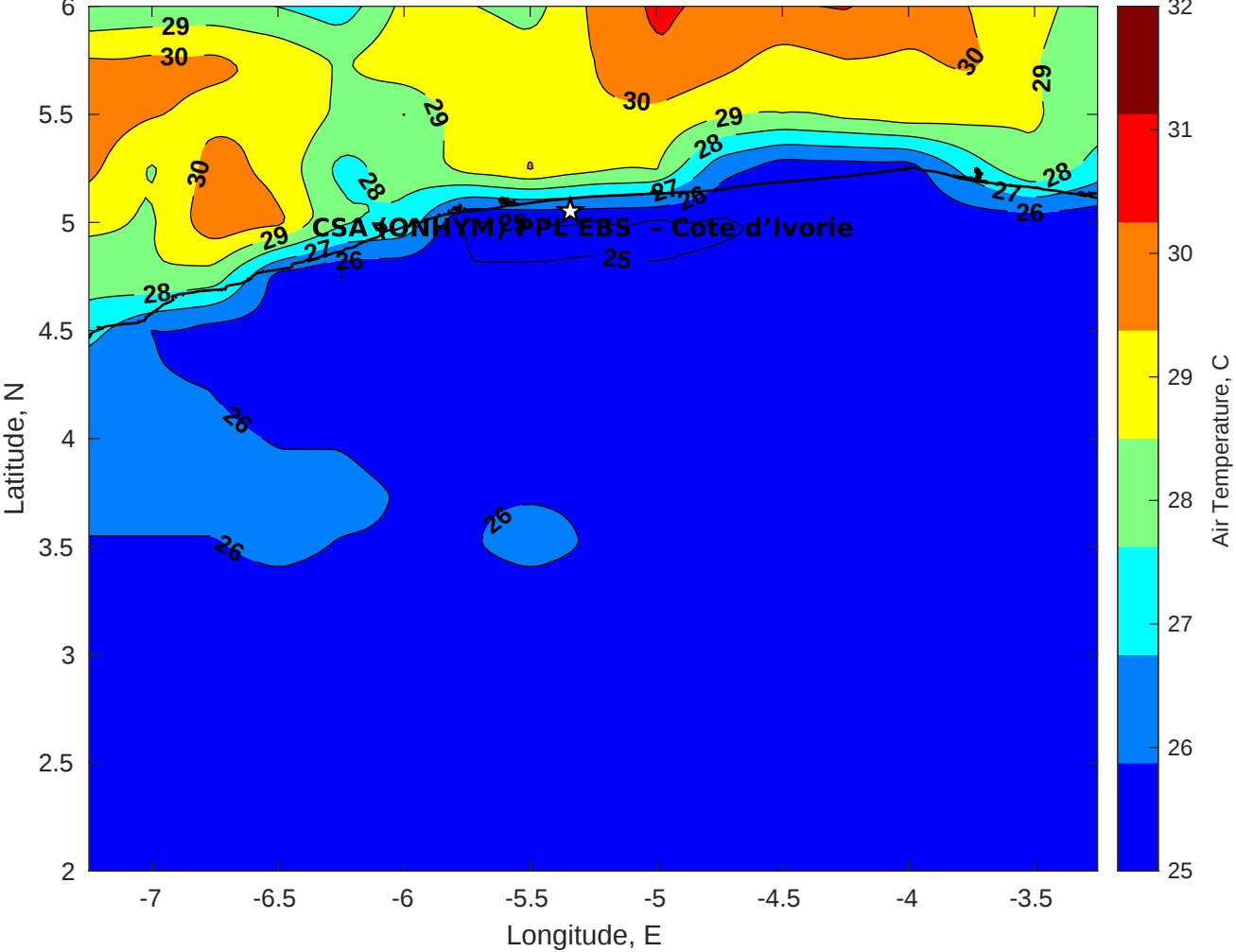
Air Temperature (C) for CSA (ONHYM) PPL EBS - Cote d'Ivoire at 12-Sep-2025
