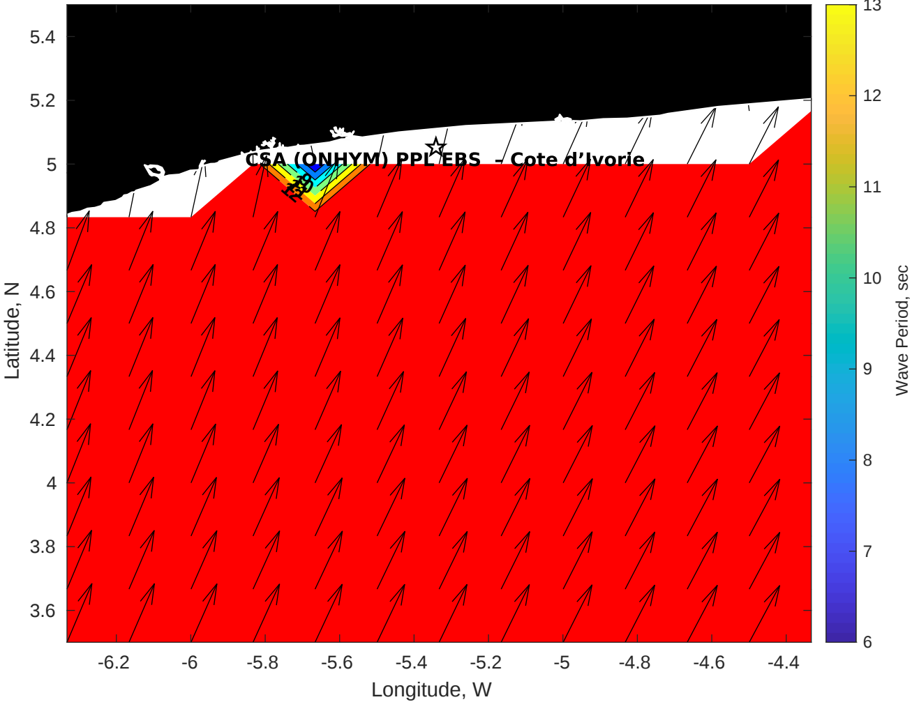
Wave Period (sec) for CSA (ONHYM) PPL EBS - Cote d'Ivoire at 13-Sep-2025 09:00:00
