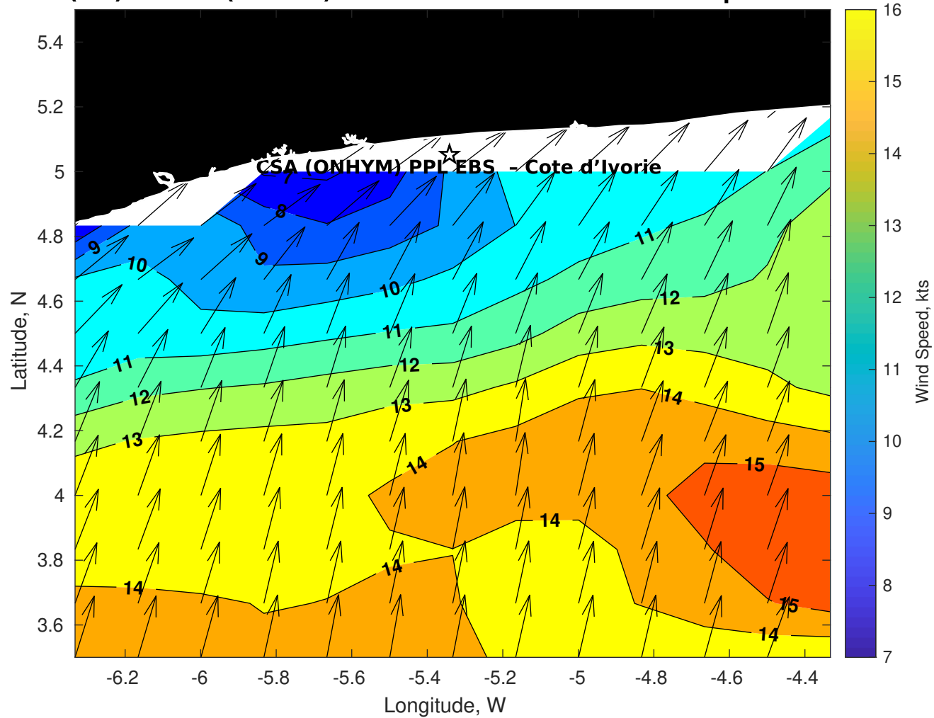
Winds (kts) for CSA (ONHYM) PPL EBS - Cote d'Ivoire at 13-Sep-2025 09:00:00
