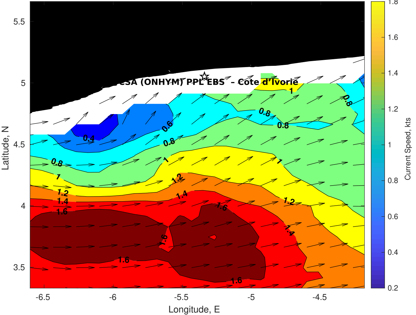
Surface Currents for CSA (ONHYM) PPL EBS - Cote d'Ivoire at 12-Sep-2025 00:00:00
