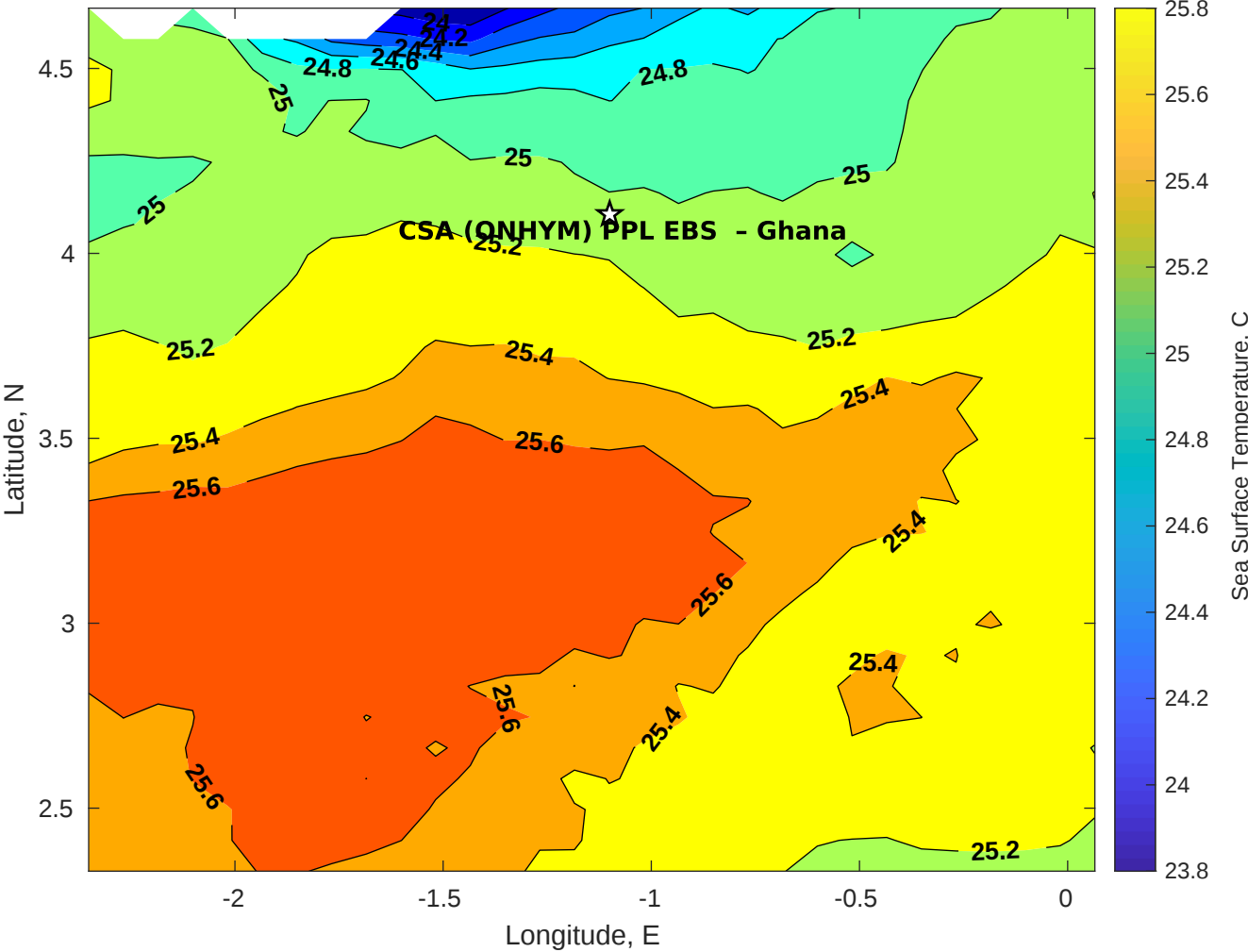
SST for CSA (ONHYM) PPL EBS - Ghana at 12-Sep-2025 00:00:00
