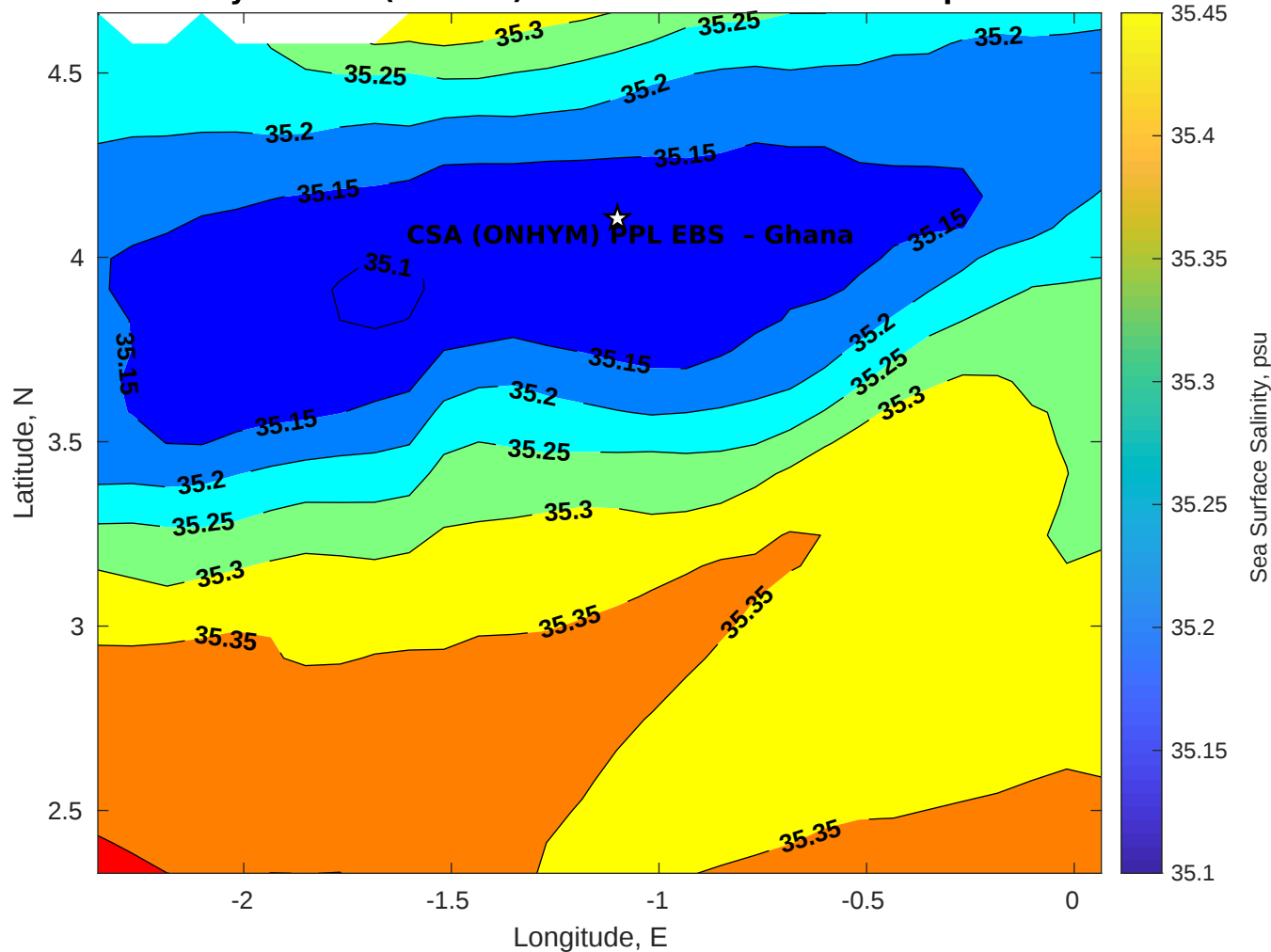
Surface Salinity for CSA (ONHYM) PPL EBS - Ghana at 12-Sep-2025 00:00:00
