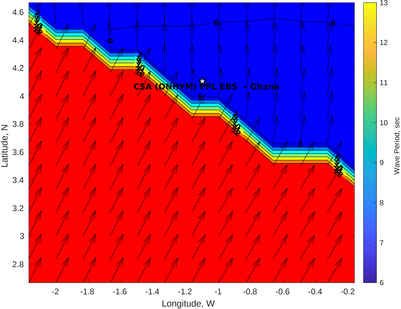
Wave Period (sec) for CSA (ONHYM) PPL EBS - Ghana at 13-Sep-2025 09:00:00
