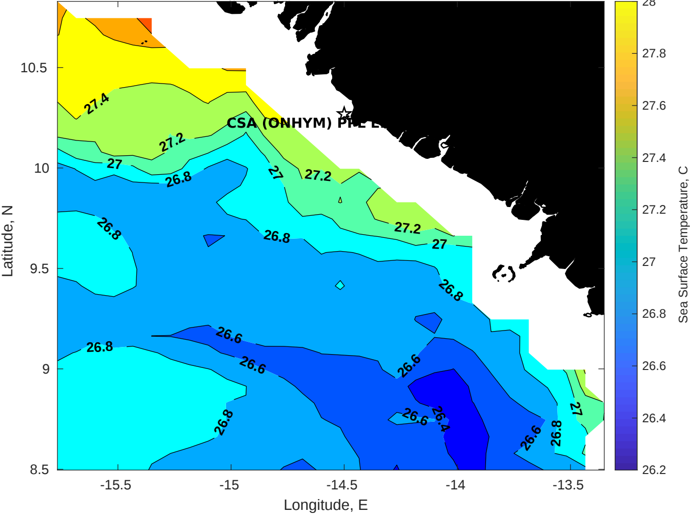
SST for CSA (ONHYM) PPL EBS - Guinea at 12-Sep-2025 00:00:00
