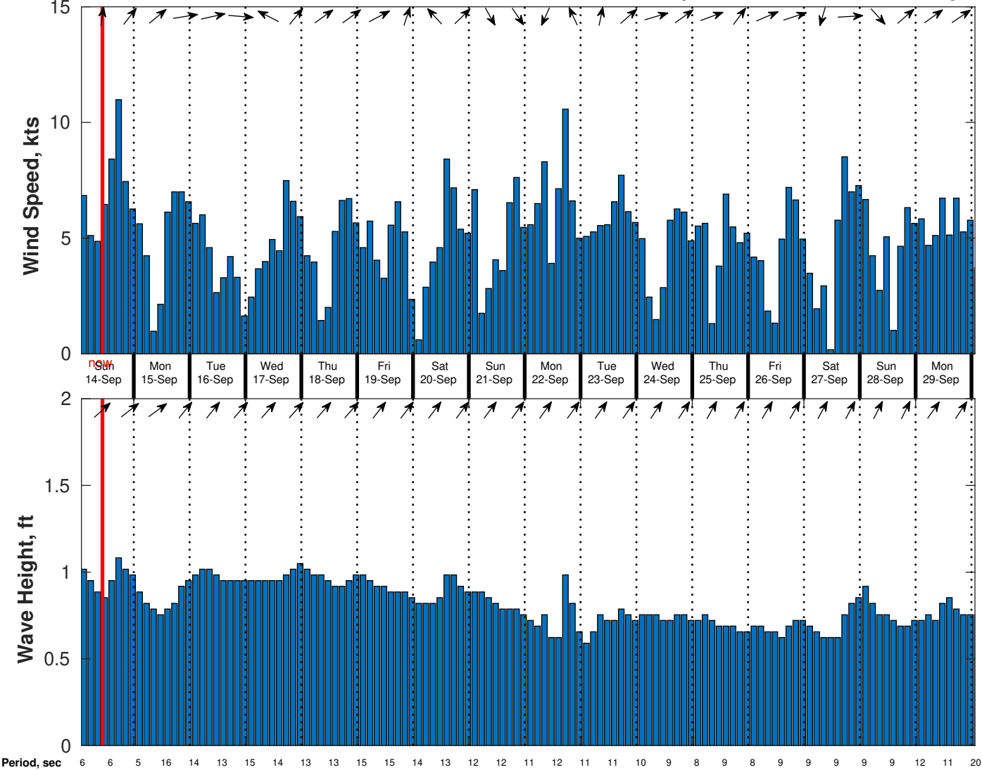
Wind & Wave Forecast for CSA (ONHYM) PPL EBS - Guinea from 13-Sep-2025 01:00:00 to 29-Sep-2025 01:00:00
