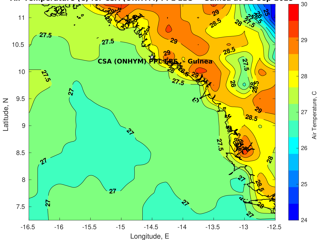
Air Temperature (C) for CSA (ONHYM) PPL EBS - Guinea at 12-Sep-2025
