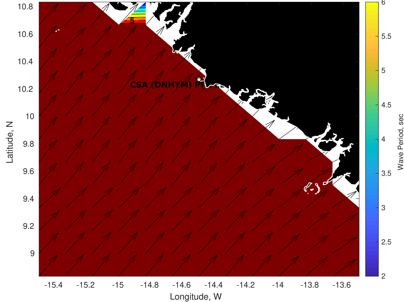
Wave Period (sec) for CSA (ONHYM) PPL EBS - Guinea at 13-Sep-2025 09:00:00
