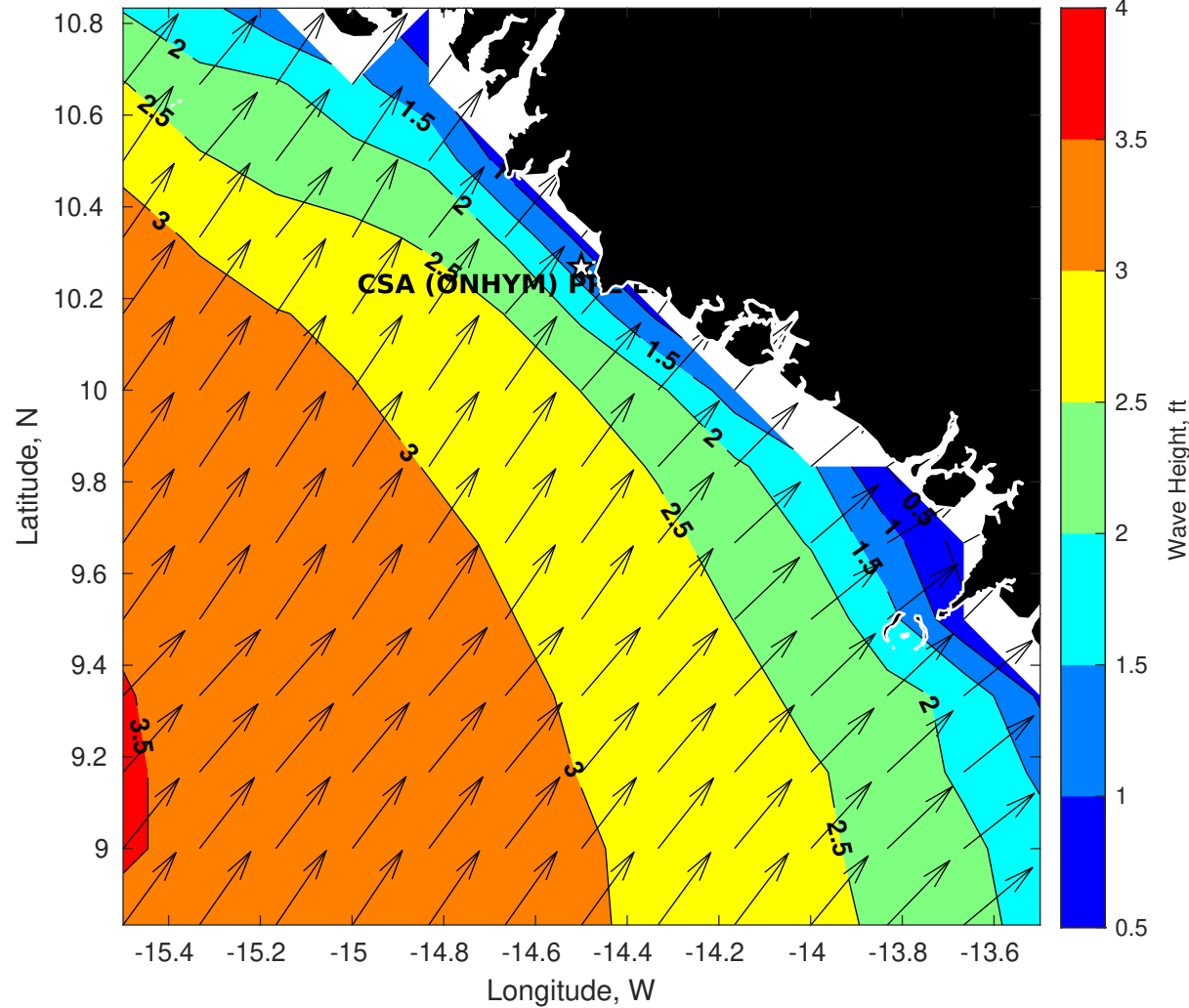
Wave Height (ft) for CSA (ONHYM) PPL EBS - Guinea at 13-Sep-2025 09:00:00
