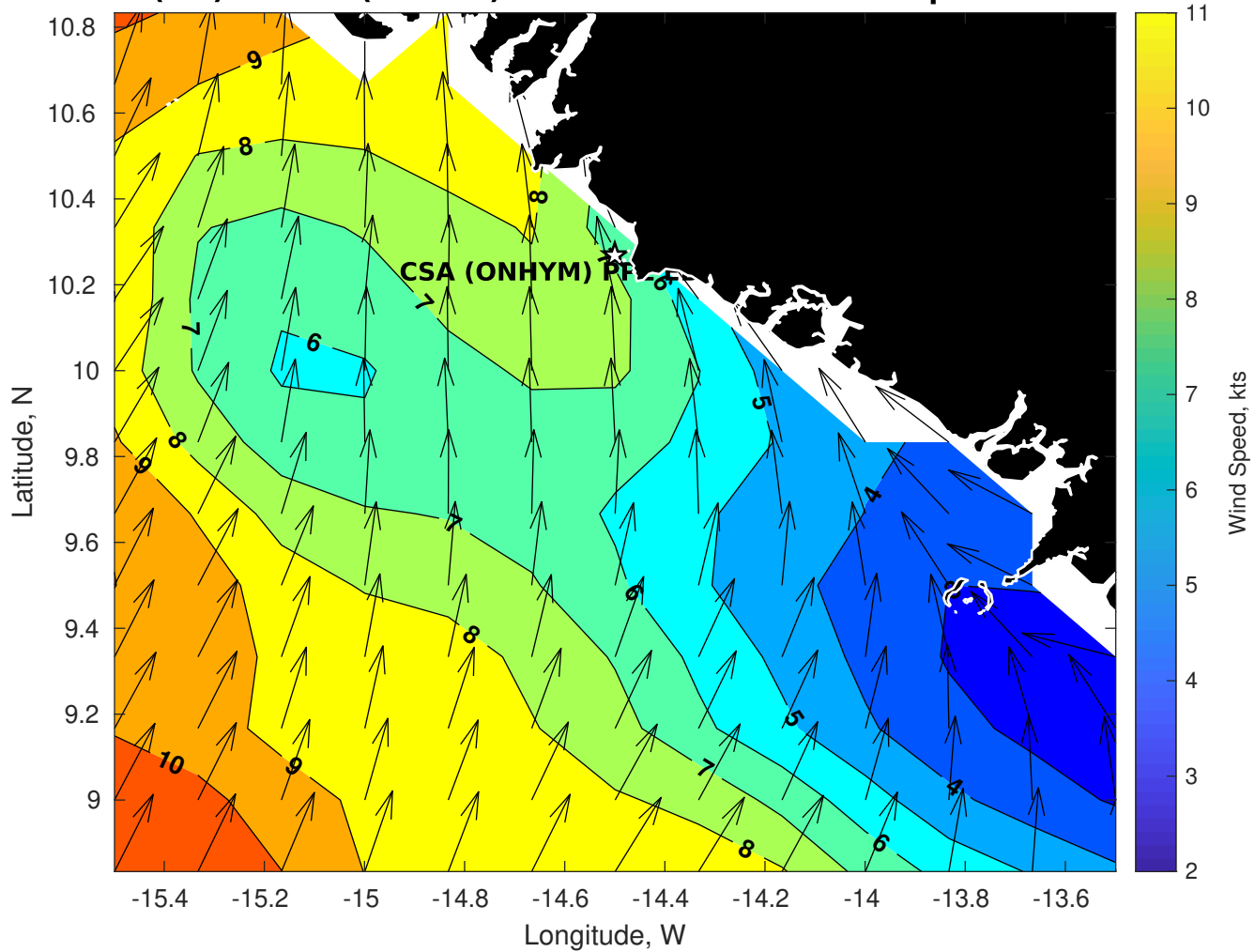
Winds (kts) for CSA (ONHYM) PPL EBS - Guinea at 13-Sep-2025 09:00:00
