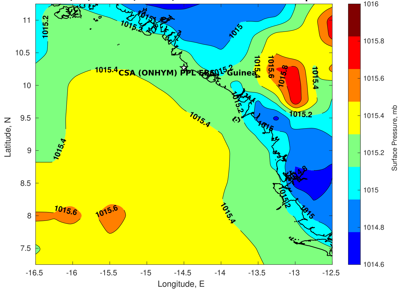
Surface Pressure (mb) for CSA (ONHYM) PPL EBS - Guinea at 14-Sep-2025 12:00:00
