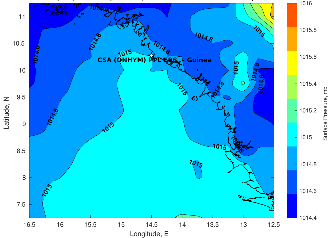
Surface Pressure (mb) for CSA (ONHYM) PPL EBS - Guinea at 13-Sep-2025 12:00:00
