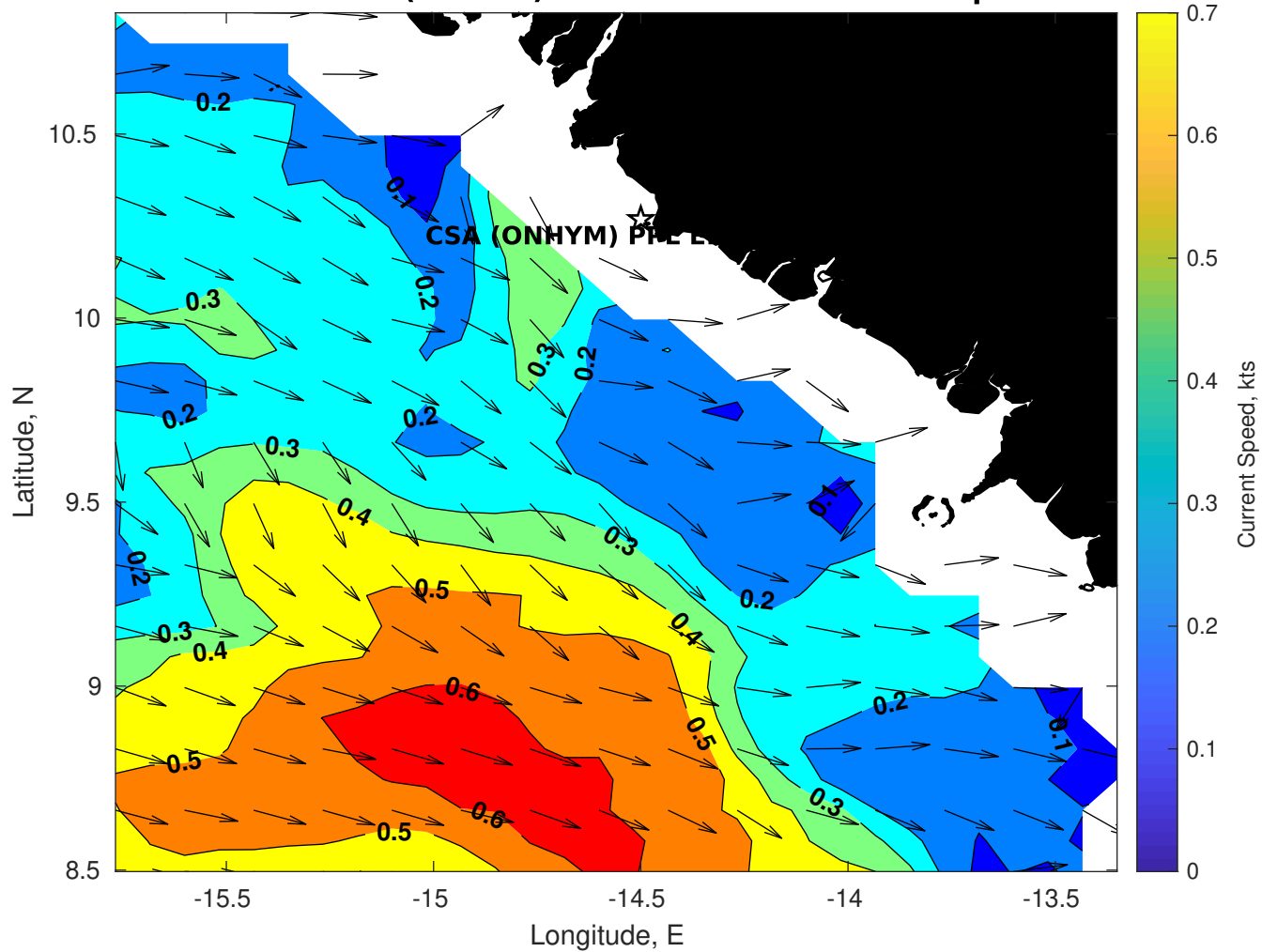
Surface Currents for CSA (ONHYM) PPL EBS - Guinea at 12-Sep-2025 00:00:00
