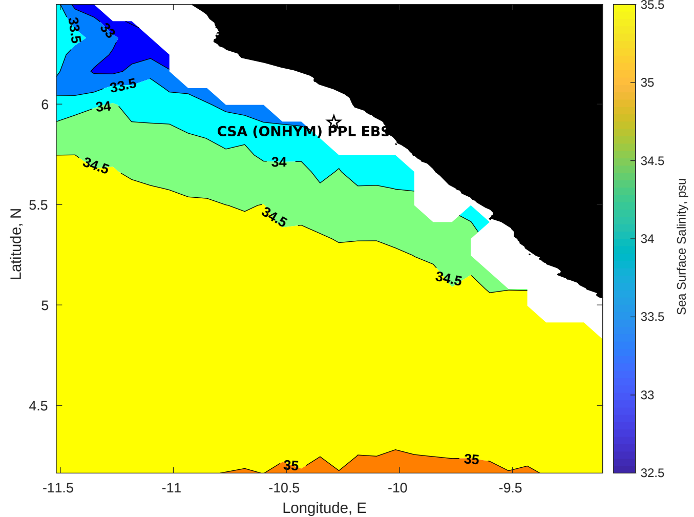
Surface Salinity for CSA (ONHYM) PPL EBS - Liberia at 12-Sep-2025 00:00:00
