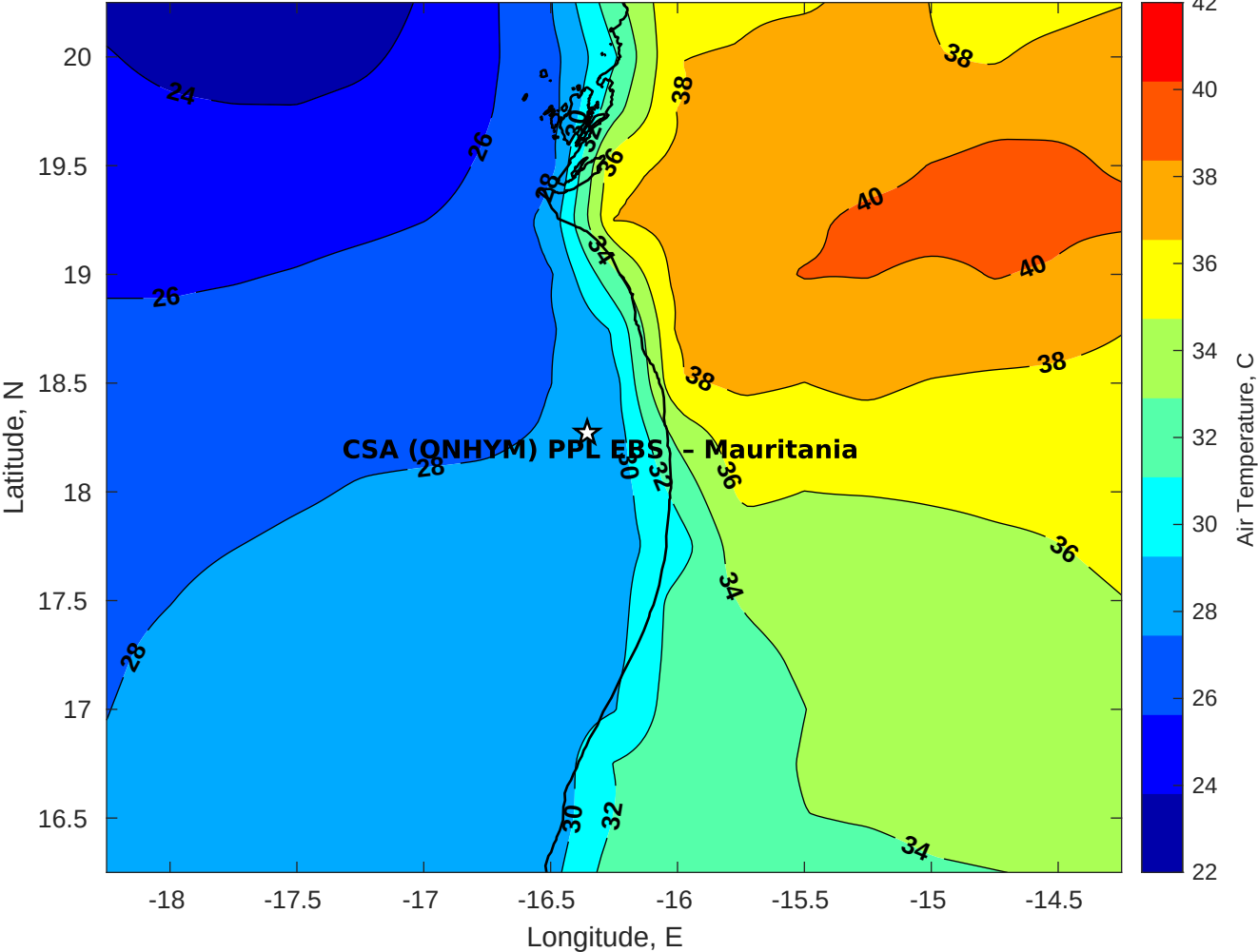
Air Temperature (C) for CSA (ONHYM) PPL EBS - Mauritania at 12-Sep-2025
