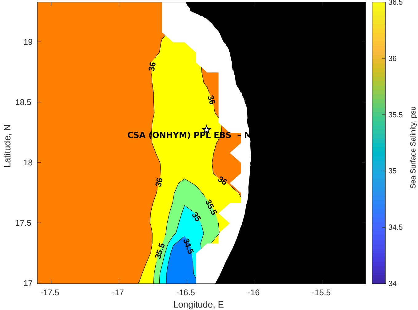
Surface Salinity for CSA (ONHYM) PPL EBS - Mauritania at 12-Sep-2025 00:00:00
