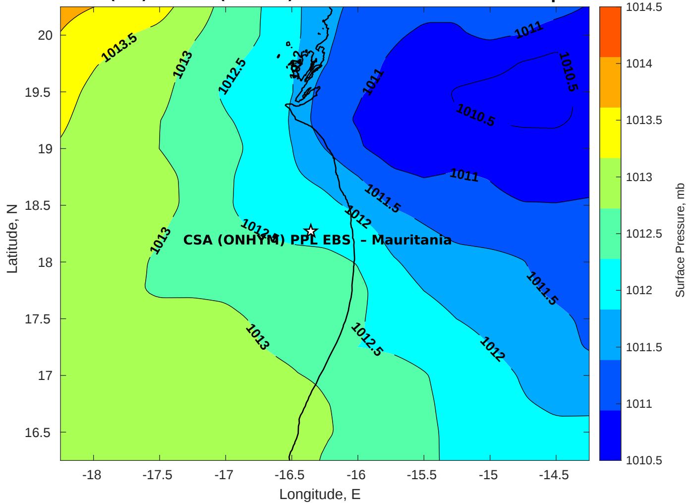
Surface Pressure (mb) for CSA (ONHYM) PPL EBS - Mauritania at 13-Sep-2025 12:00:00
