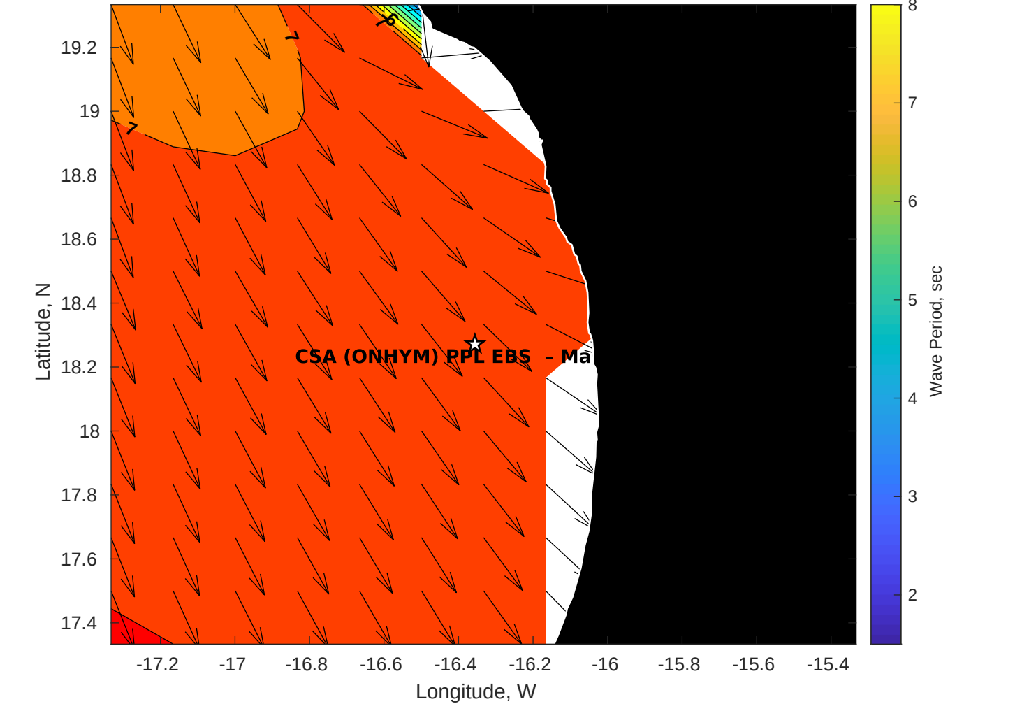
Wave Period (sec) for CSA (ONHYM) PPL EBS - Mauritania at 13-Sep-2025 09:00:00
