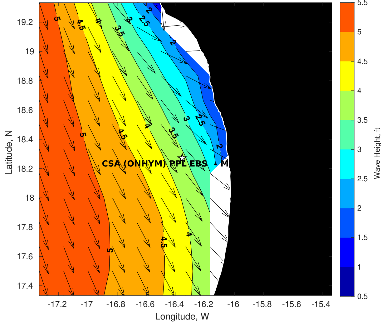
Wave Height (ft) for CSA (ONHYM) PPL EBS - Mauritania at 13-Sep-2025 09:00:00
