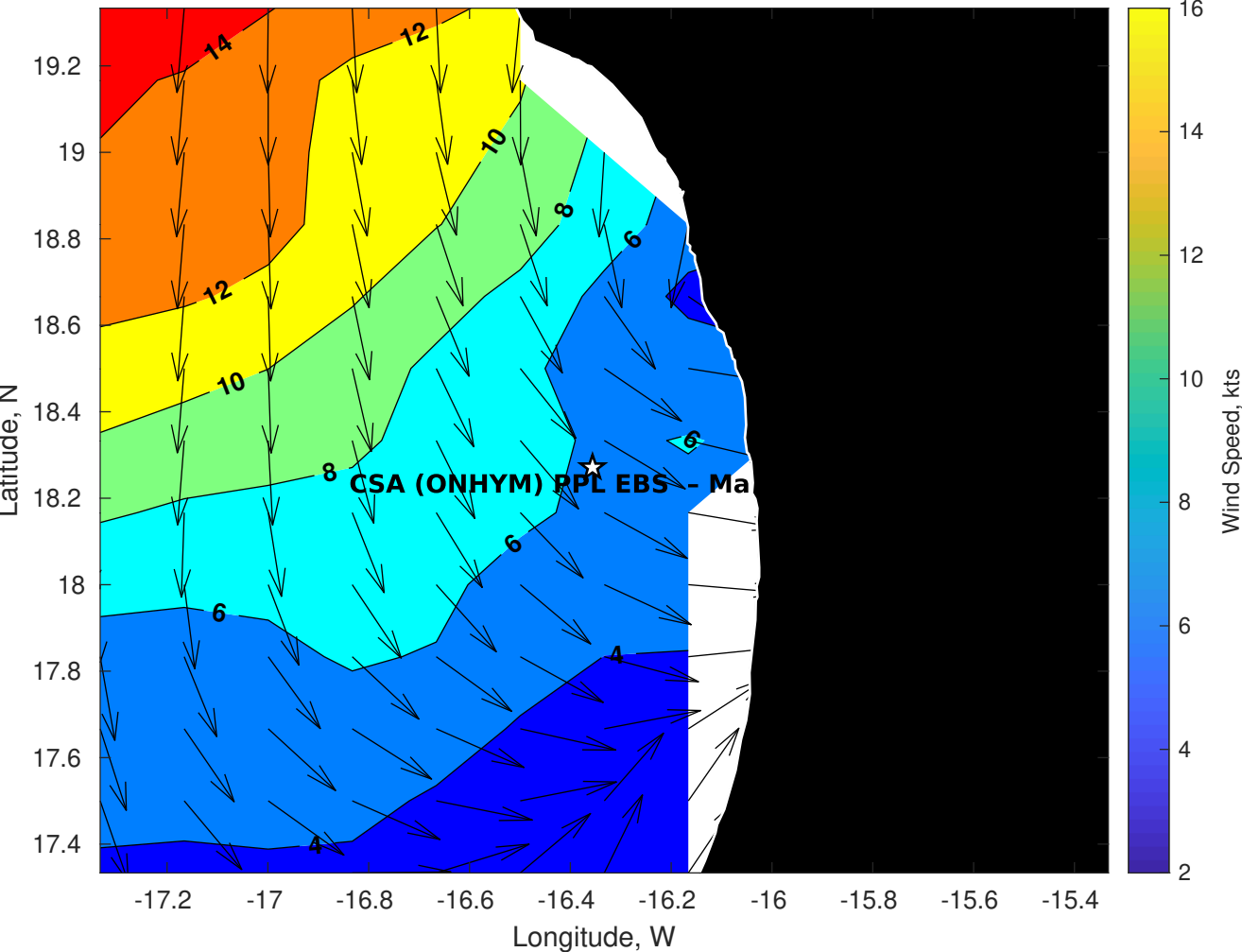
Winds (kts) for CSA (ONHYM) PPL EBS - Mauritania at 13-Sep-2025 09:00:00
