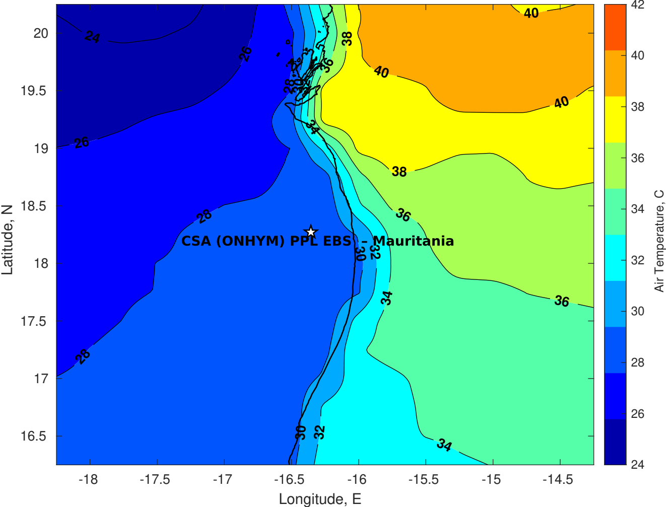
Air Temperature (C) for CSA (ONHYM) PPL EBS - Mauritania at 12-Sep-2025
