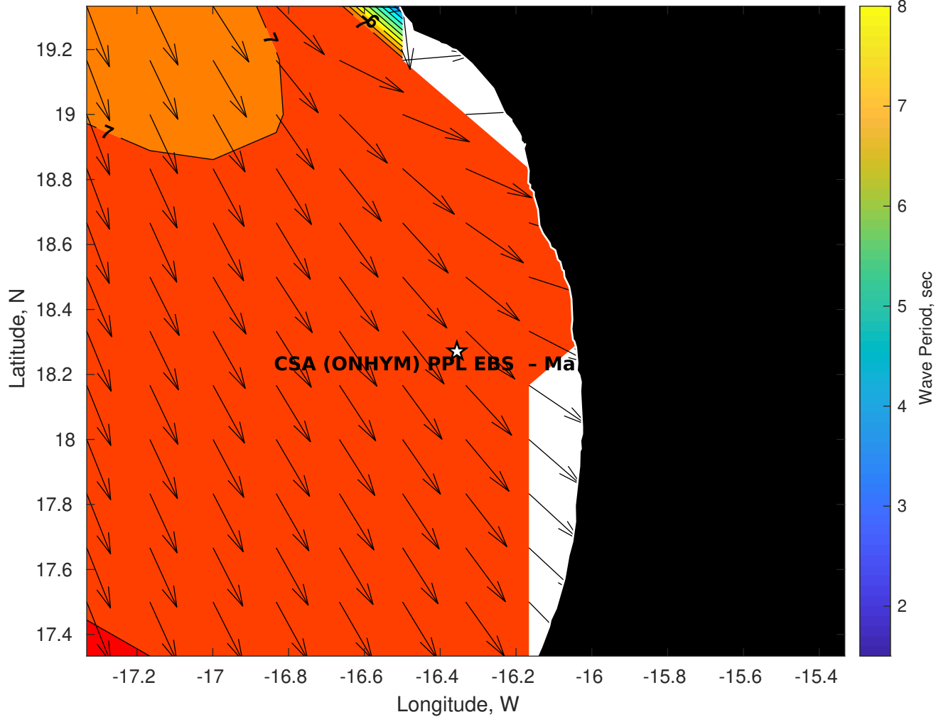
Wave Period (sec) for CSA (ONHYM) PPL EBS - Mauritania at 13-Sep-2025 09:00:00
