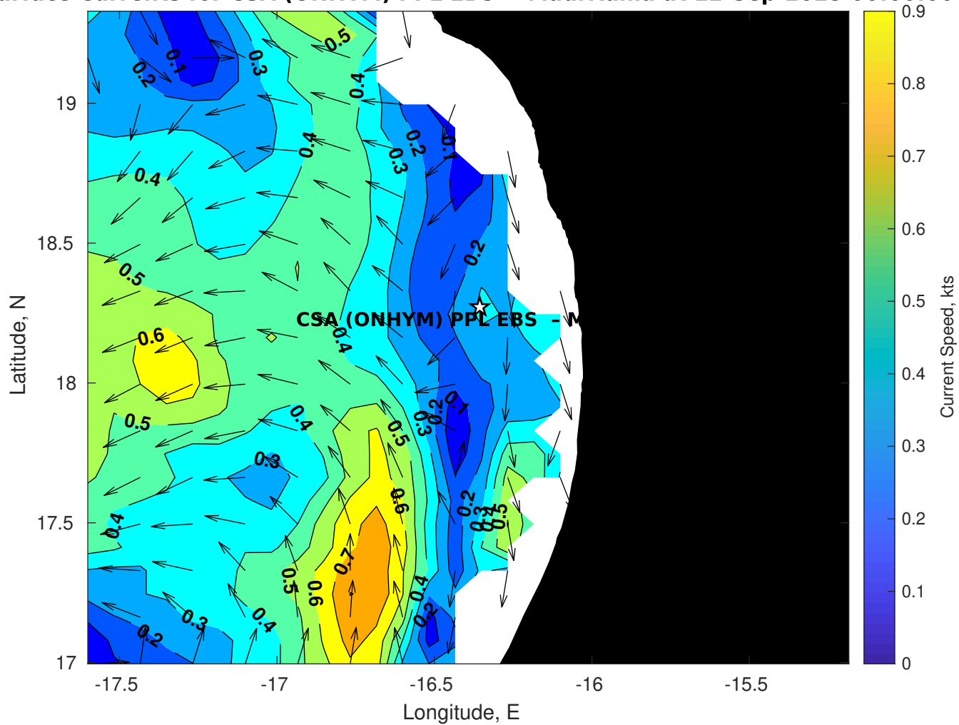
Surface Currents for CSA (ONHYM) PPL EBS - Mauritania at 12-Sep-2025 00:00:00
