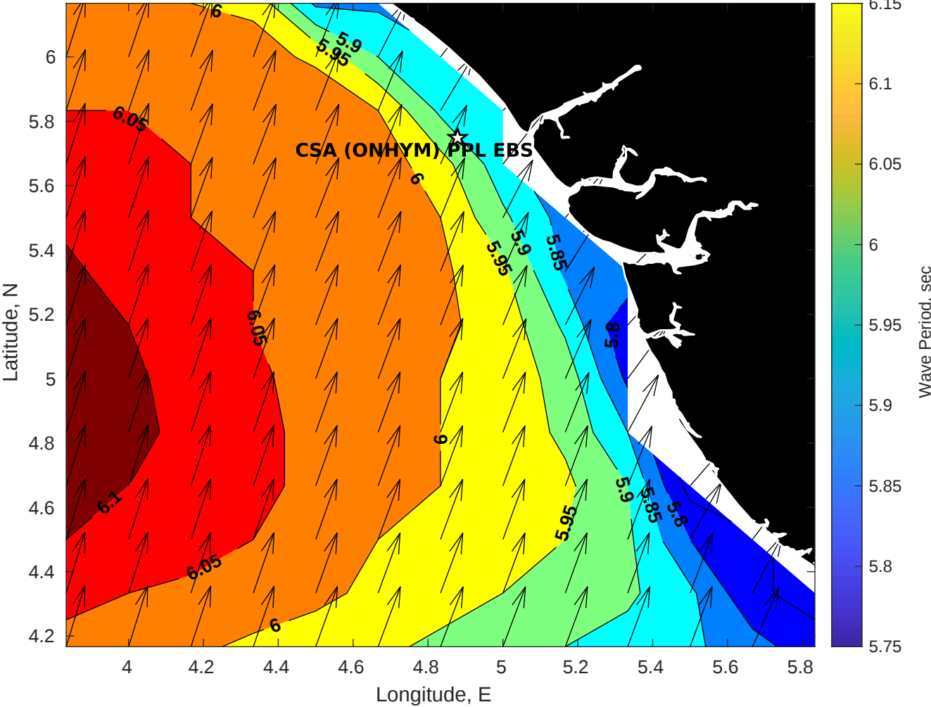
Wave Period (sec) for CSA (ONHYM) PPL EBS - Nigeria at 13-Sep-2025 09:00:00
