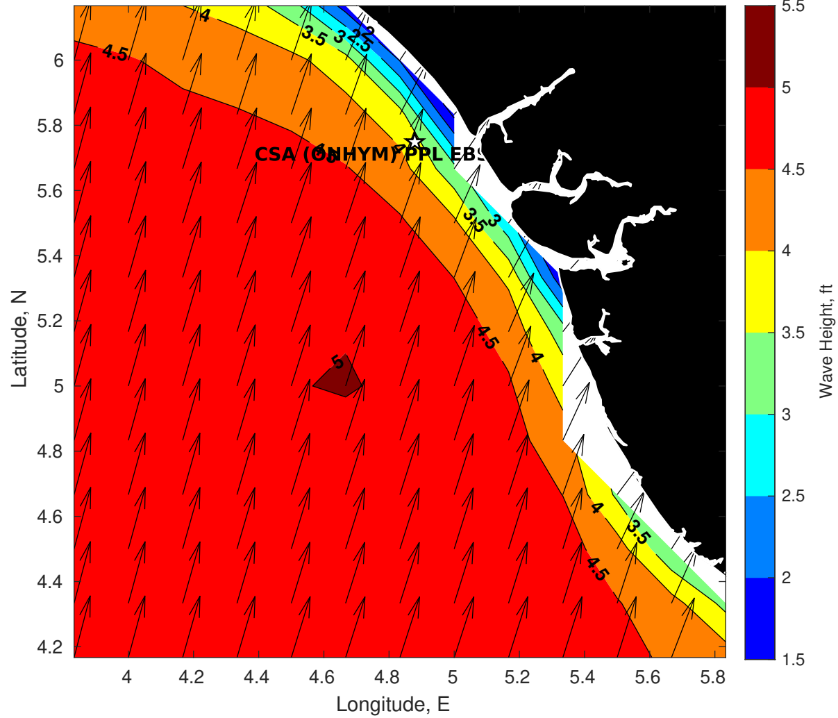
Wave Height (ft) for CSA (ONHYM) PPL EBS - Nigeria at 13-Sep-2025 09:00:00
