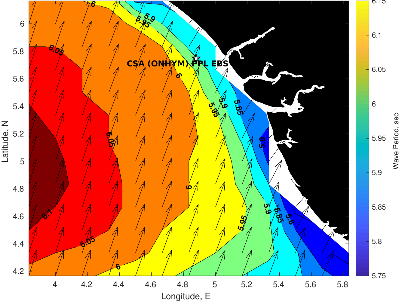
Wave Period (sec) for CSA (ONHYM) PPL EBS - Nigeria at 13-Sep-2025 09:00:00
