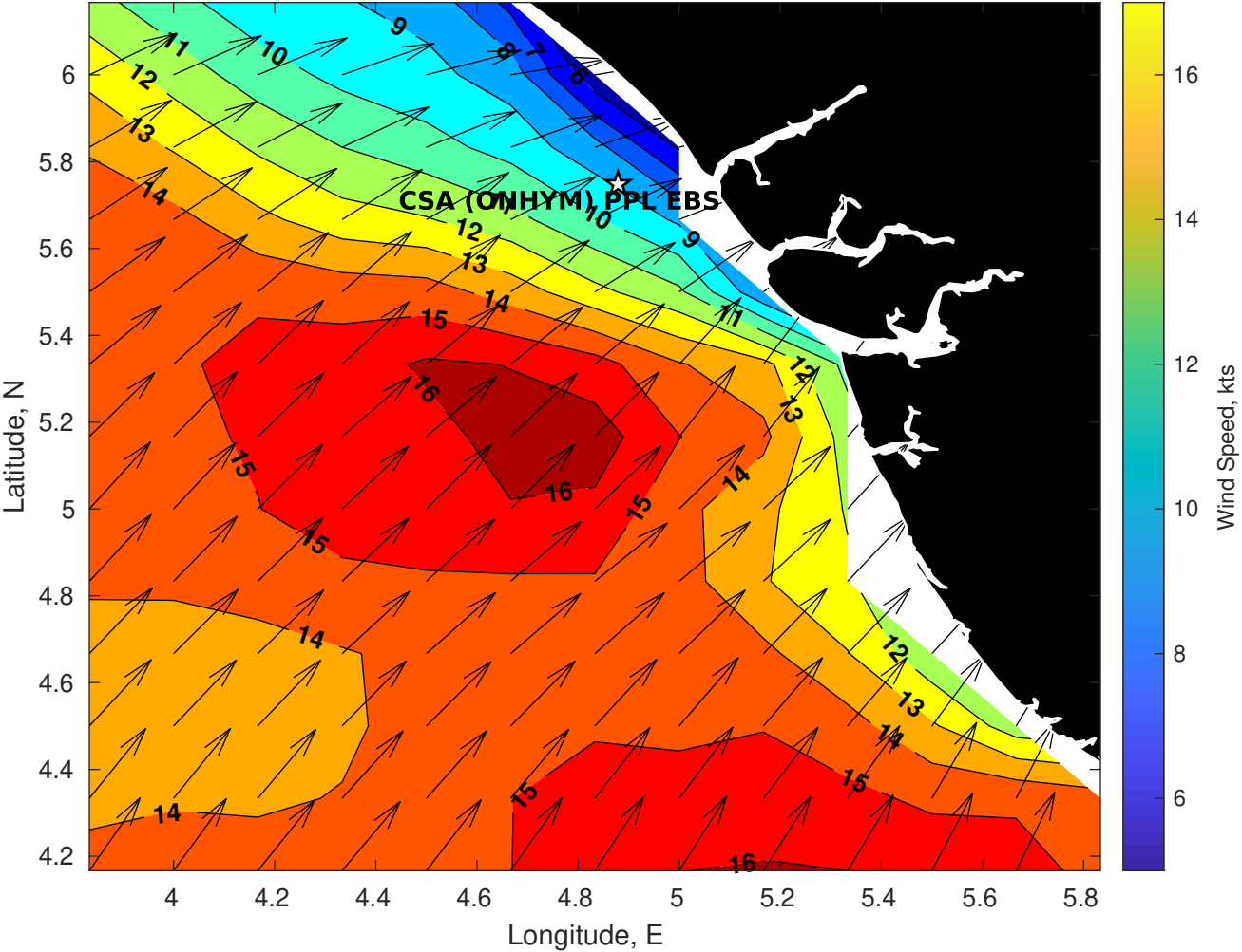
Winds (kts) for CSA (ONHYM) PPL EBS - Nigeria at 13-Sep-2025 09:00:00
