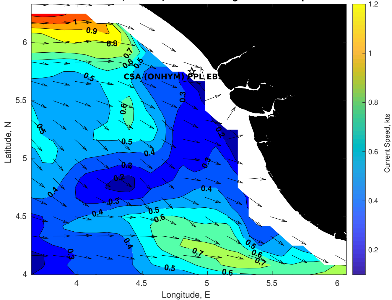
Surface Currents for CSA (ONHYM) PPL EBS - Nigeria at 12-Sep-2025 00:00:00
