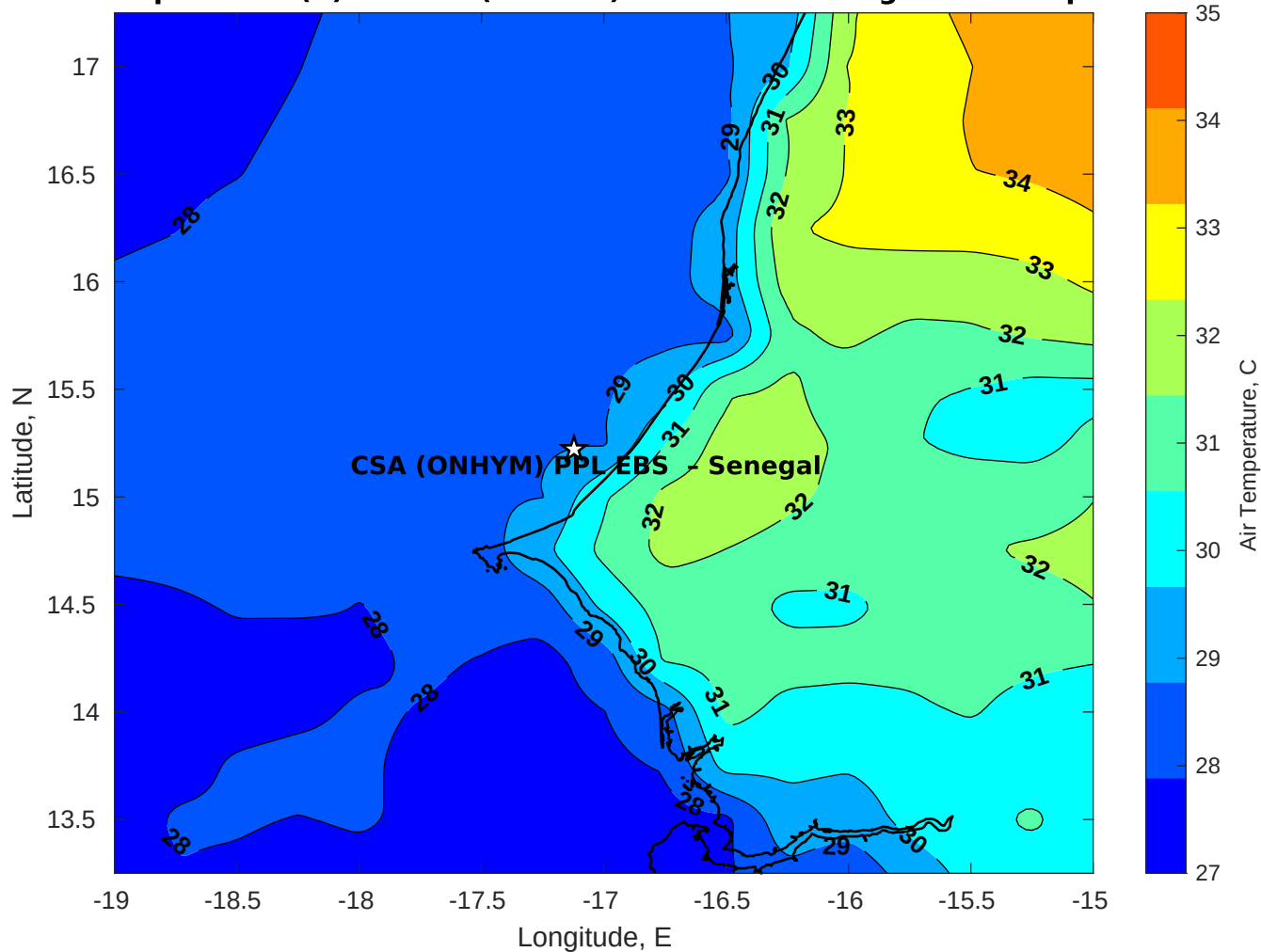
Air Temperature (C) for CSA (ONHYM) PPL EBS - Senegal at 12-Sep-2025
