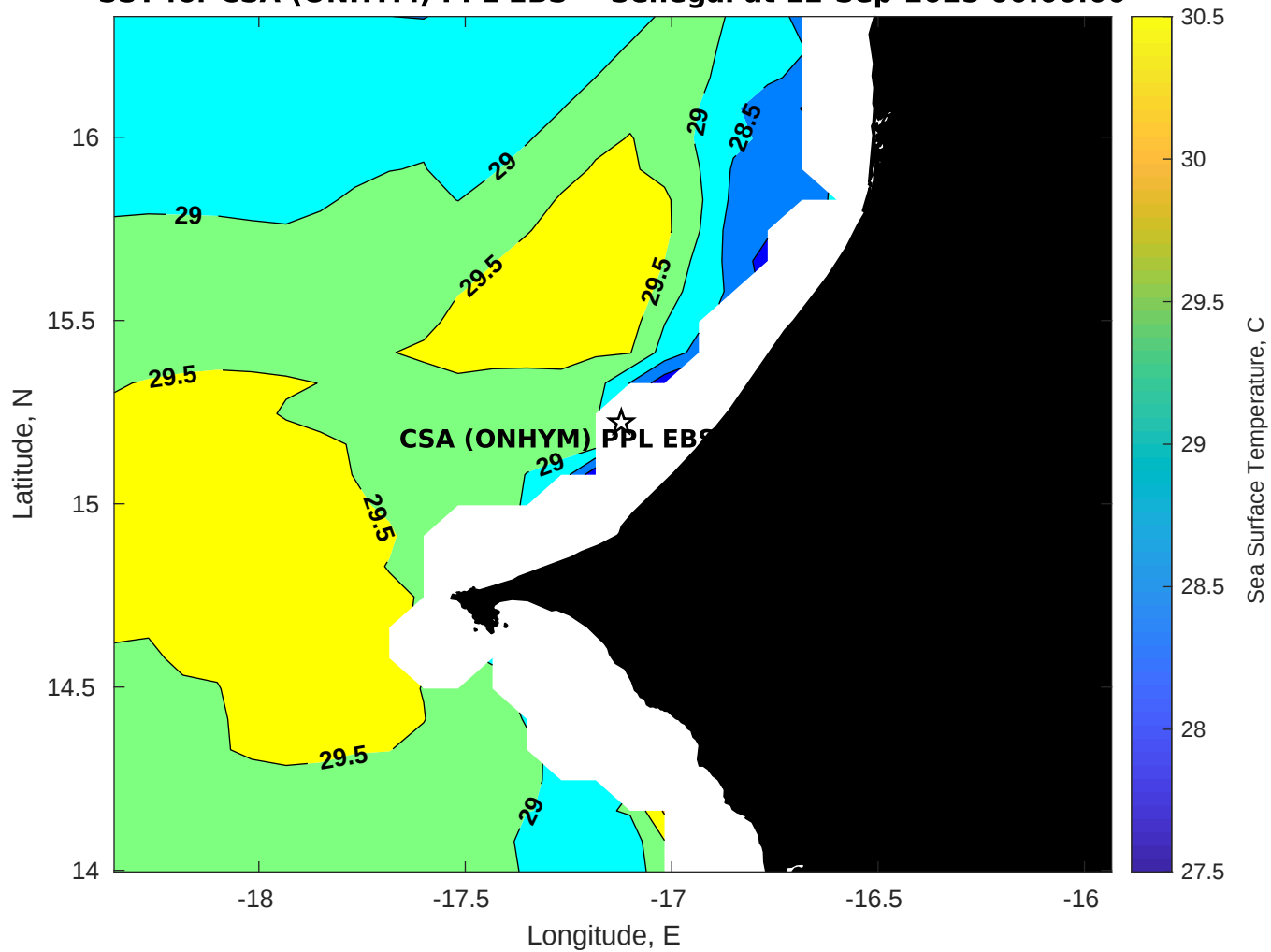
SST for CSA (ONHYM) PPL EBS - Senegal at 12-Sep-2025 00:00:00
