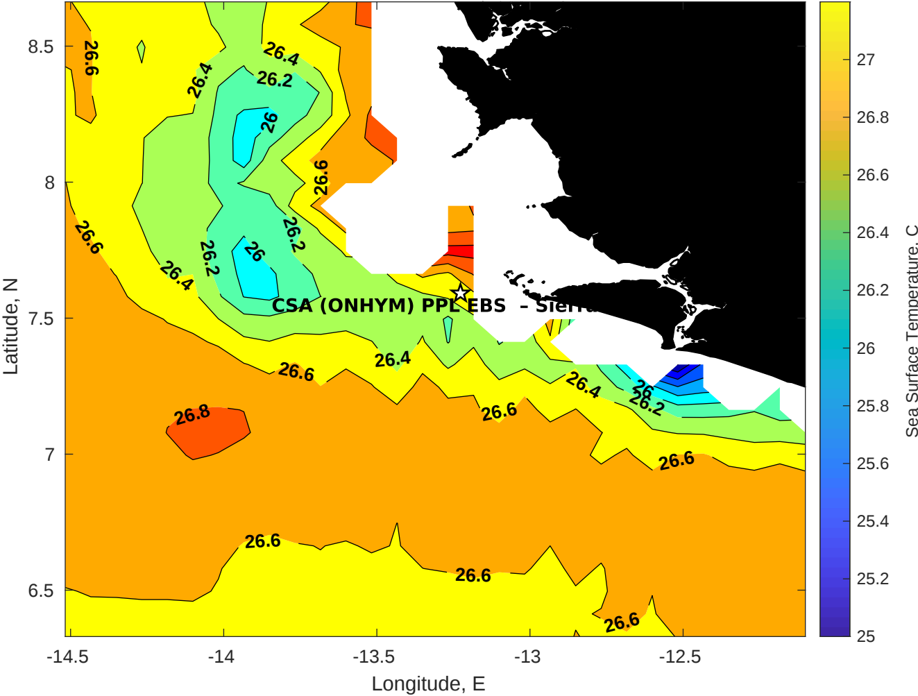
SST for CSA (ONHYM) PPL EBS - Sierra Leone at 12-Sep-2025 00:00:00
