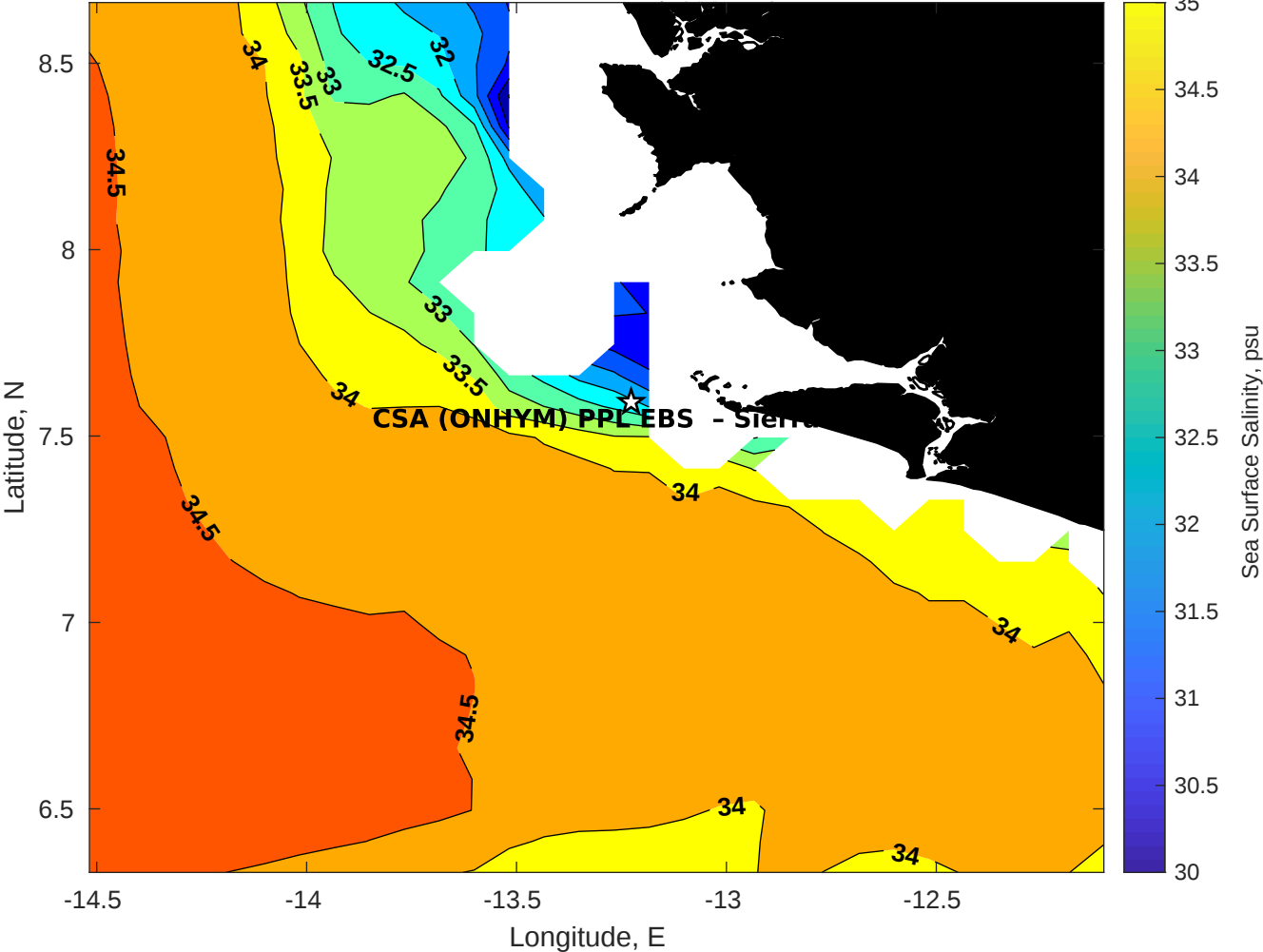
Surface Salinity for CSA (ONHYM) PPL EBS - Sierra Leone at 12-Sep-2025 00:00:00
