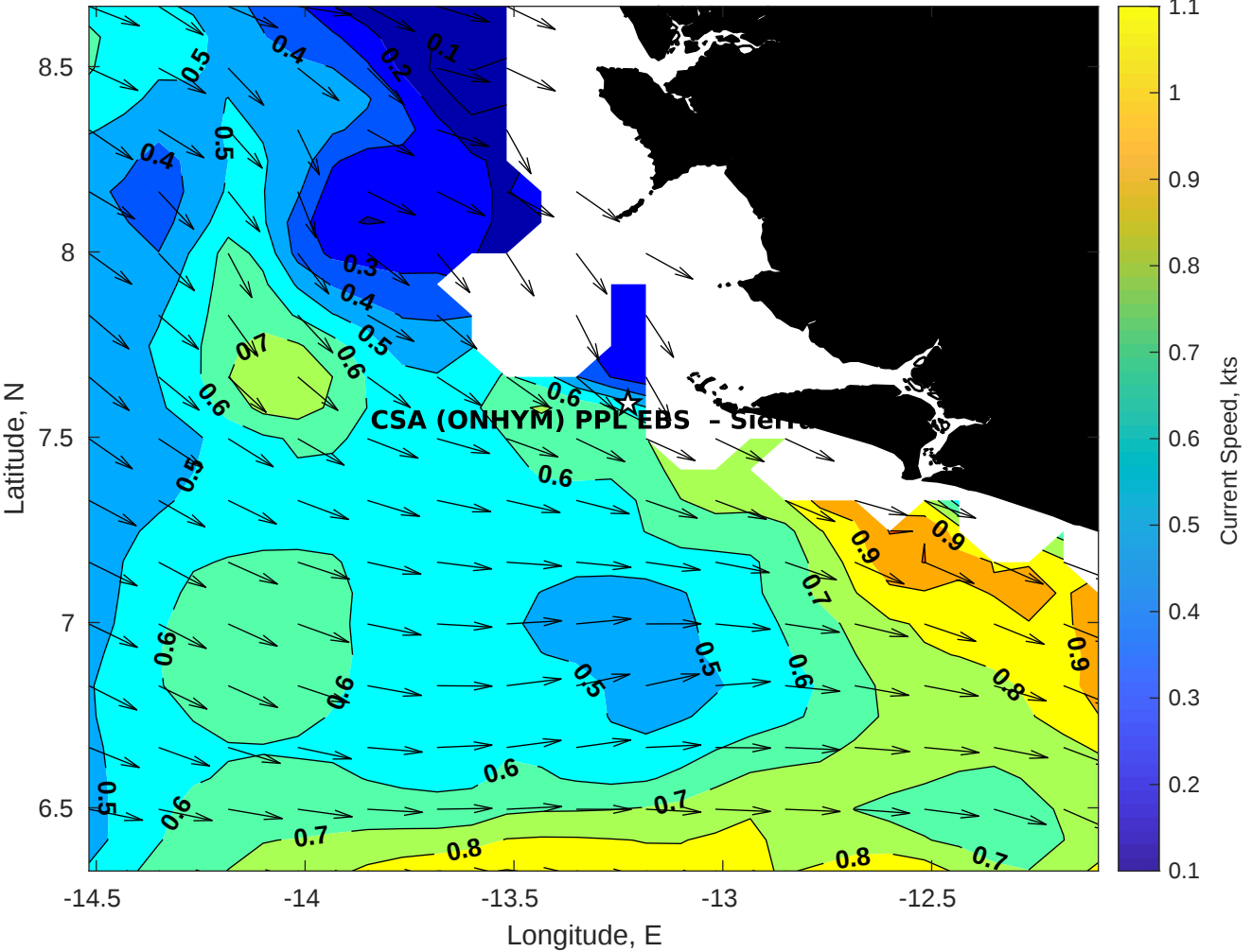
Surface Currents for CSA (ONHYM) PPL EBS - Sierra Leone at 12-Sep-2025 00:00:00
