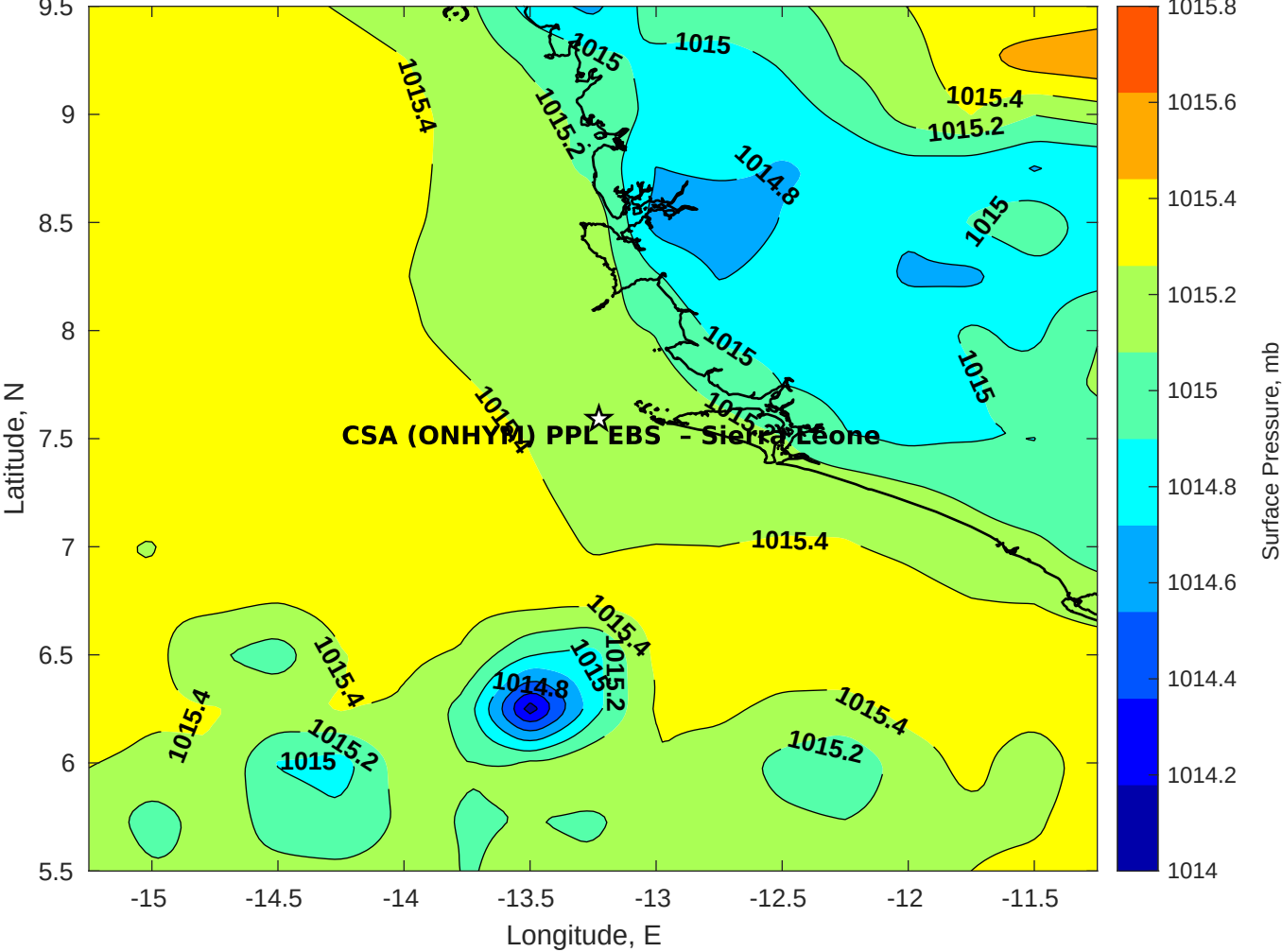
Surface Pressure (mb) for CSA (ONHYM) PPL EBS - Sierra Leone at 14-Sep-2025 12:00:00
