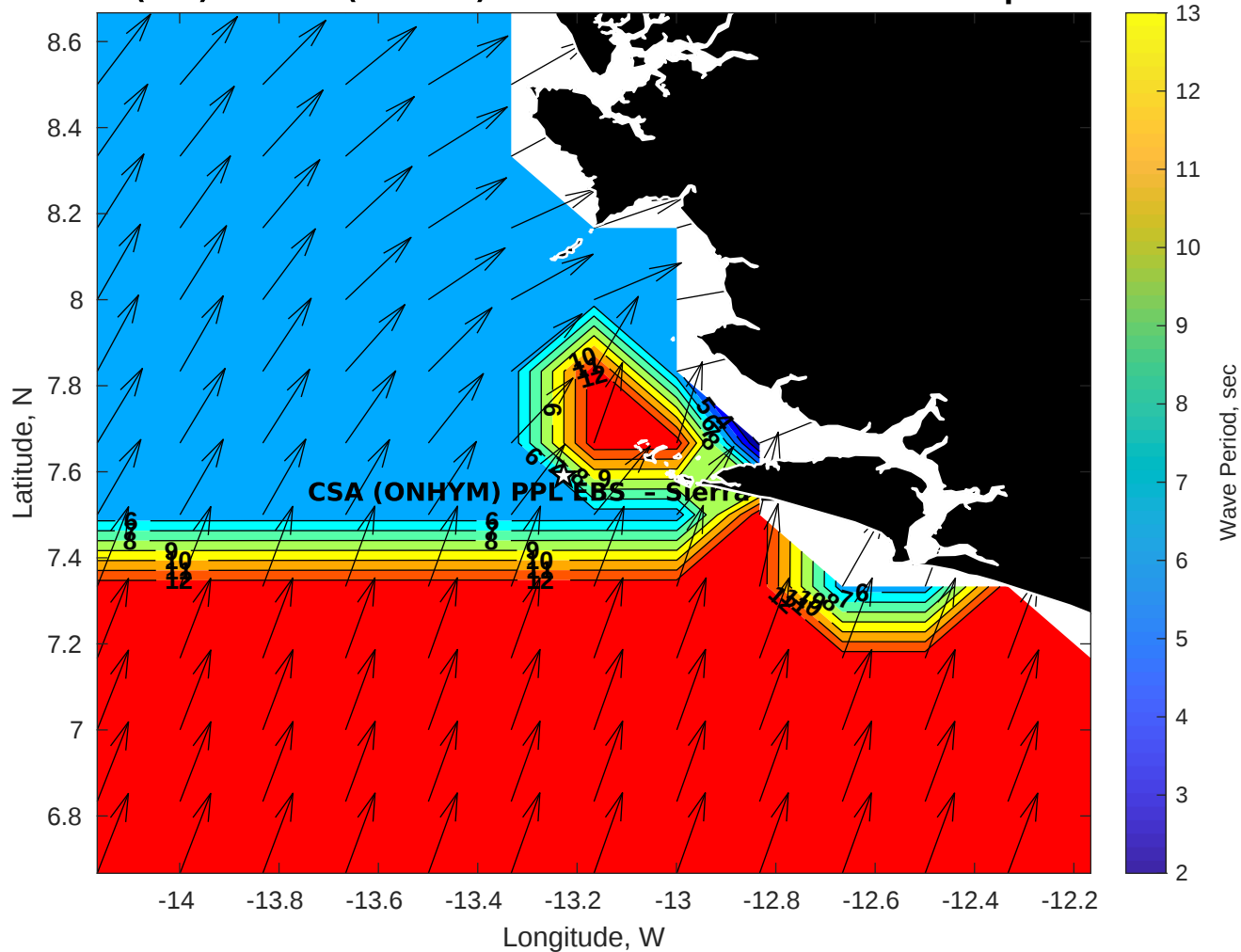
Wave Period (sec) for CSA (ONHYM) PPL EBS - Sierra Leone at 13-Sep-2025 09:00:00
