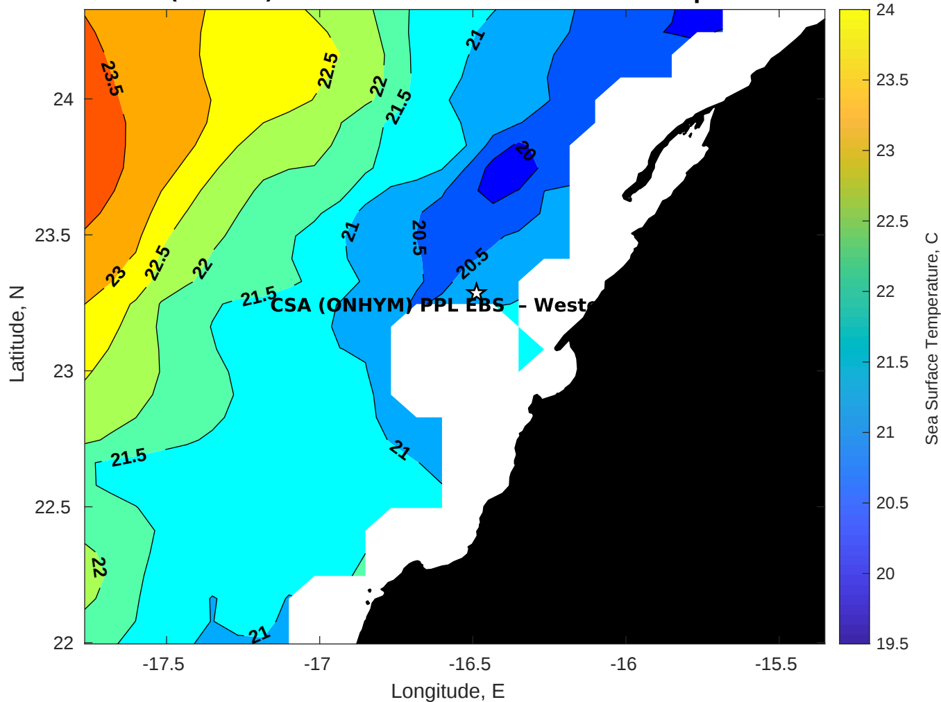
SST for CSA (ONHYM) PPL EBS - Western Sahara at 12-Sep-2025 00:00:00
