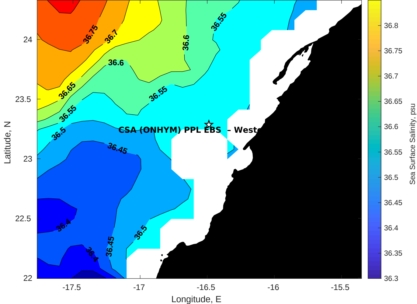
Surface Salinity for CSA (ONHYM) PPL EBS - Western Sahara at 12-Sep-2025 00:00:00
