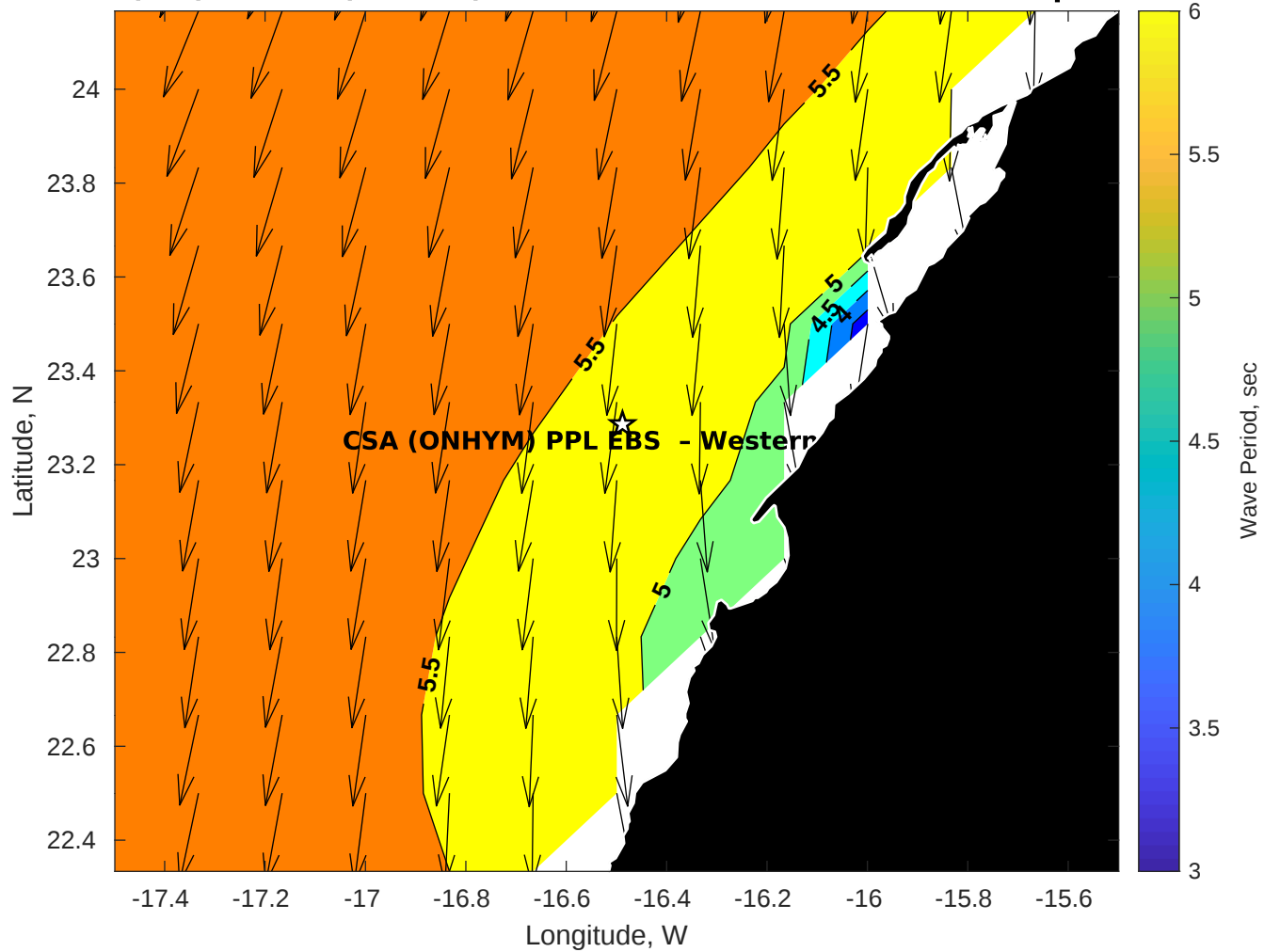
Wave Period (sec) for CSA (ONHYM) PPL EBS - Western Sahara at 13-Sep-2025 09:00:00
