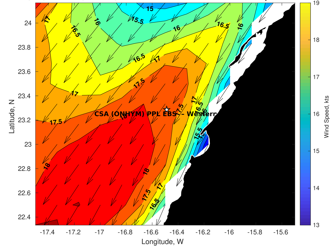
Winds (kts) for CSA (ONHYM) PPL EBS - Western Sahara at 13-Sep-2025 09:00:00
