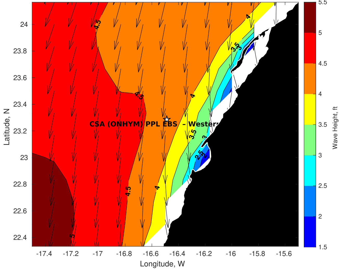
Wave Height (ft) for CSA (ONHYM) PPL EBS - Western Sahara at 13-Sep-2025 09:00:00
