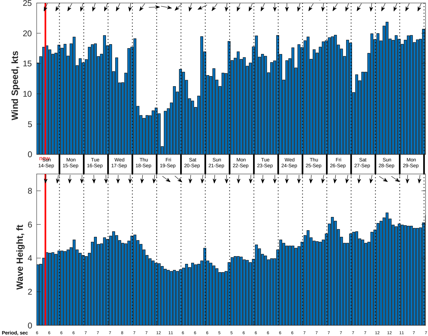
Wind & Wave Forecast for CSA (ONHYM) PPL EBS - Western Sahara from 13-Sep-2025 01:00:00 to 29-Sep-2025 01:00:00
