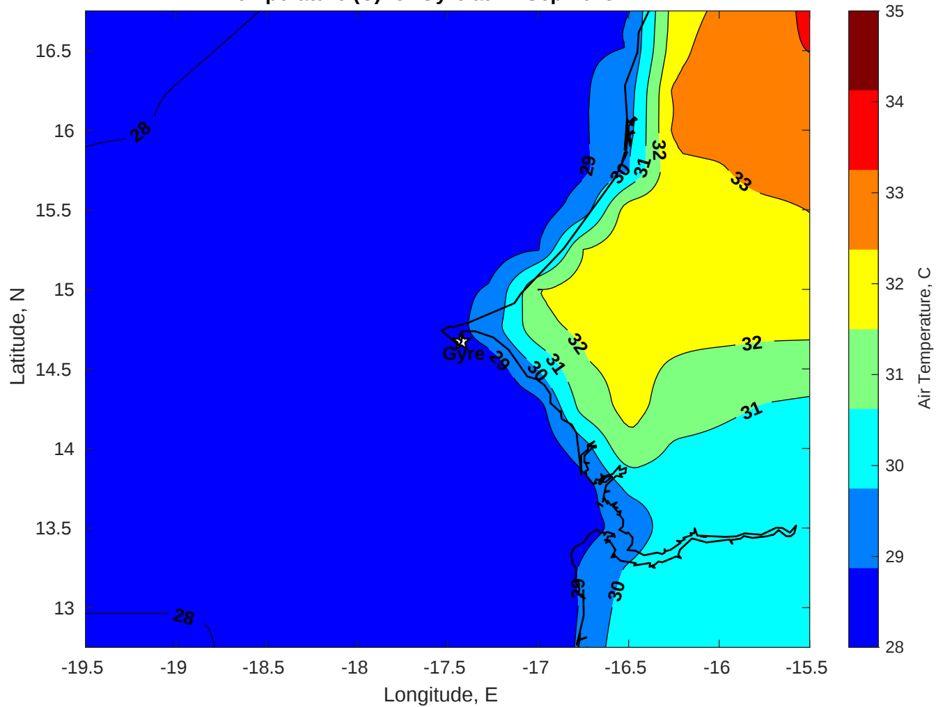
Air Temperature (C) for Gyre at 12-Sep-2025
