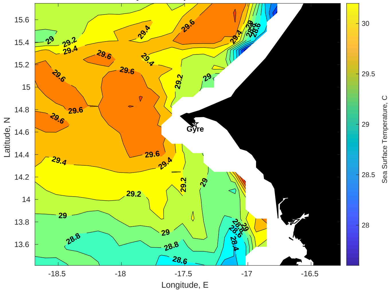
SST for Gyre at 12-Sep-2025 00:00:00
