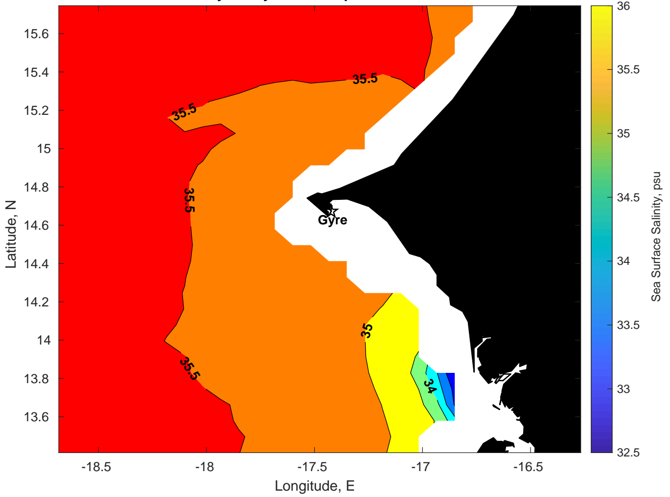
Surface Salinity for Gyre at 12-Sep-2025 00:00:00
