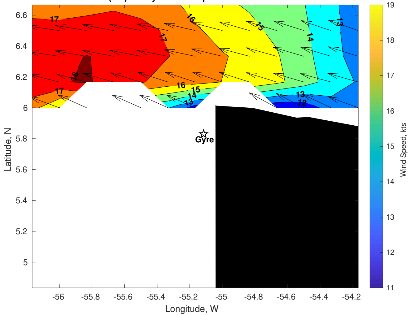
Winds (kts) for Gyre at 13-Sep-2025 09:00:00
