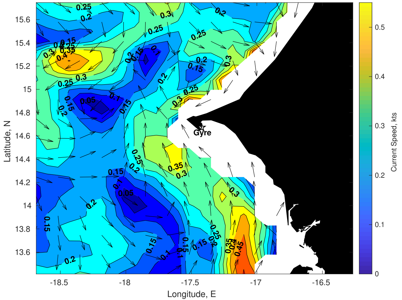
Surface Currents for Gyre at 12-Sep-2025 00:00:00
