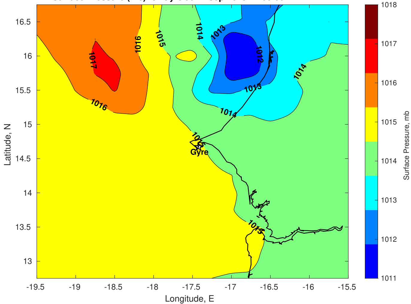
Surface Pressure (mb) for Gyre at 14-Sep-2025 12:00:00
