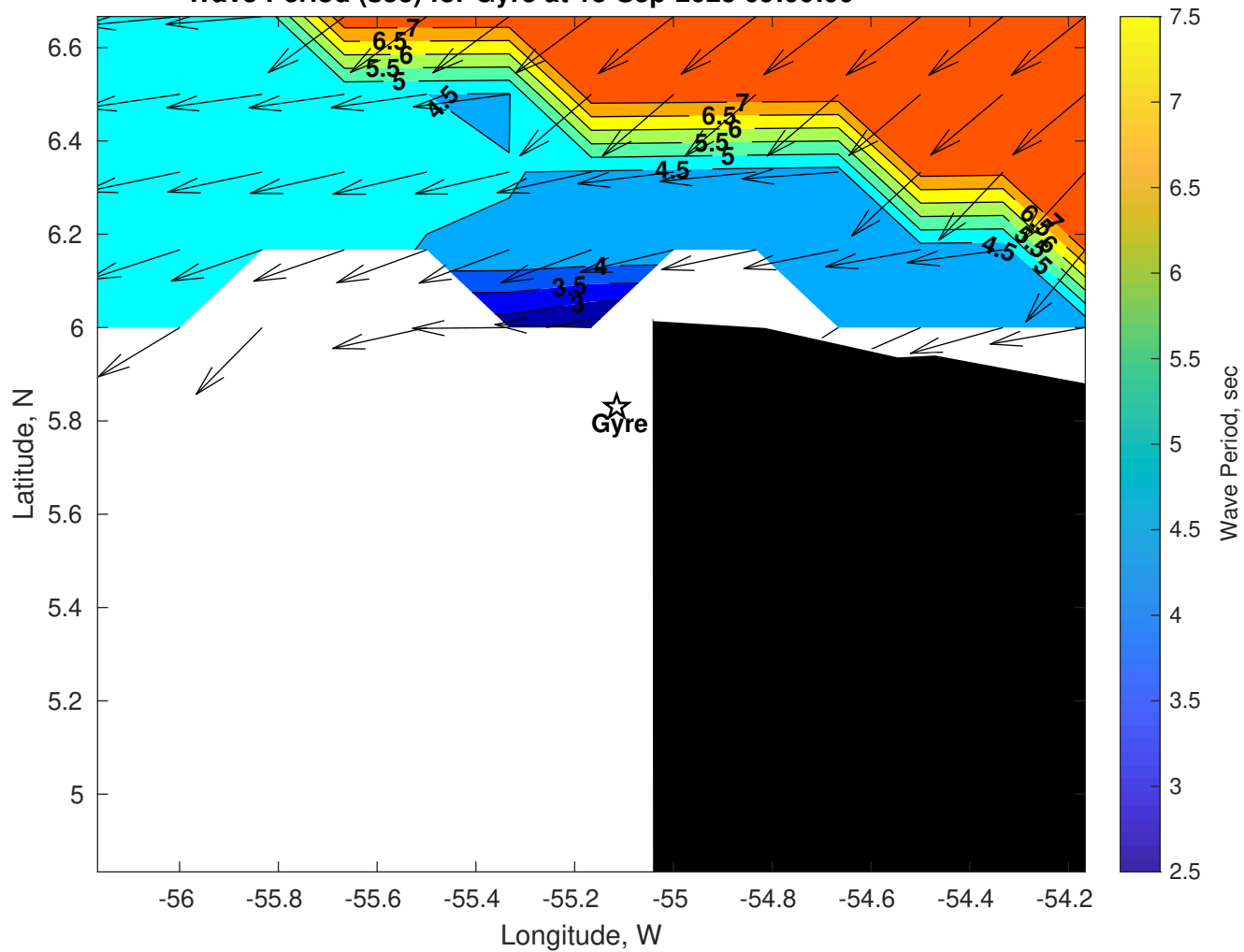
Wave Period (sec) for Gyre at 13-Sep-2025 09:00:00
