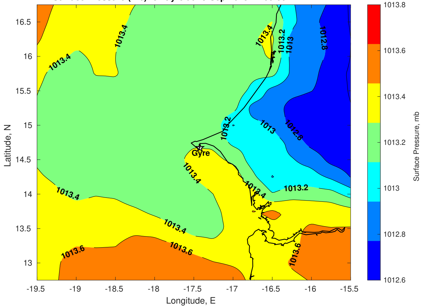
Surface Pressure (mb) for Gyre at 13-Sep-2025 12:00:00
