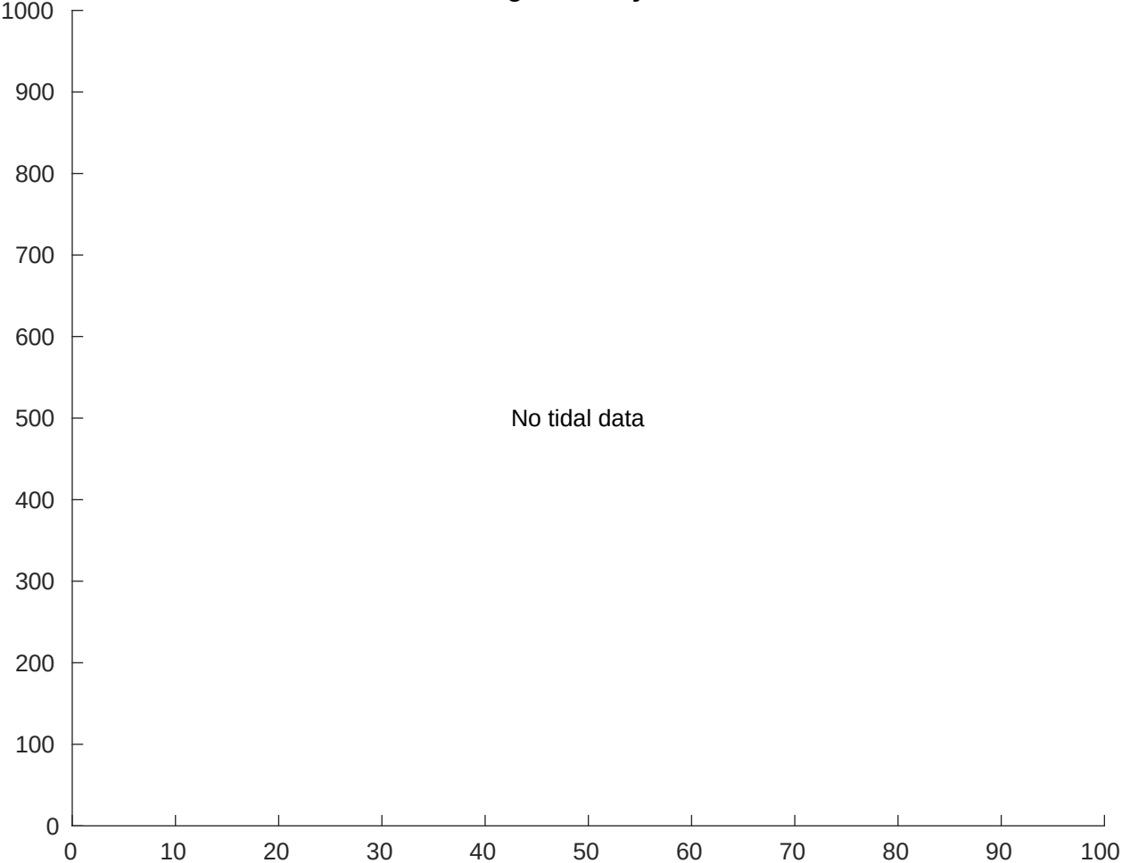
Tidal Currents and Heights for Gyre at 20250913
