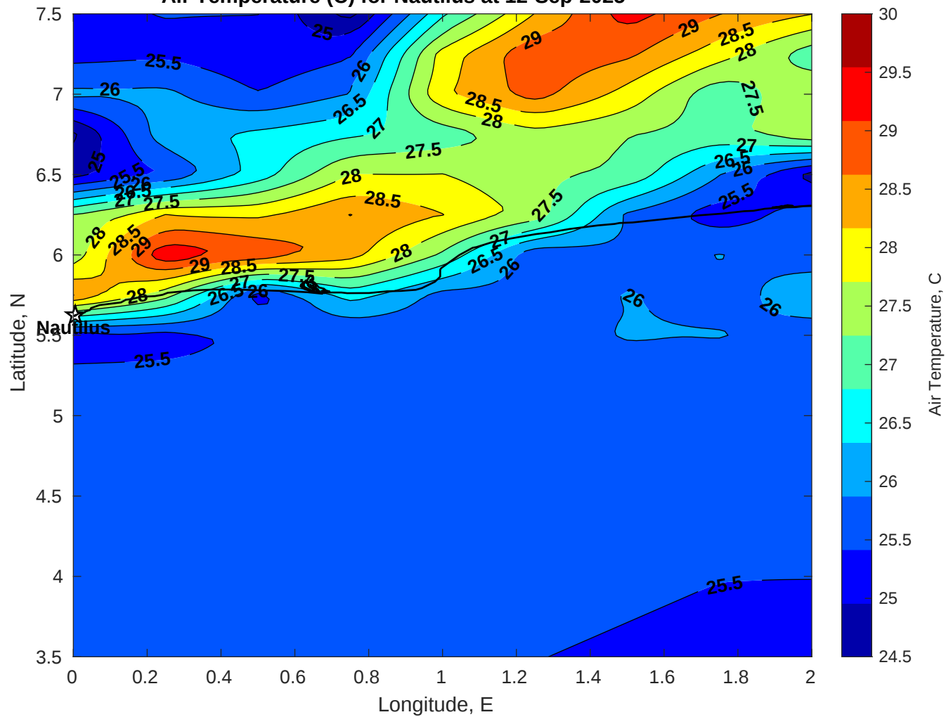
Air Temperature (C) for Nautilus at 12-Sep-2025
