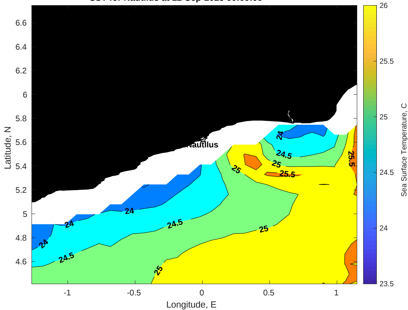
SST for Nautilus at 12-Sep-2025 00:00:00
