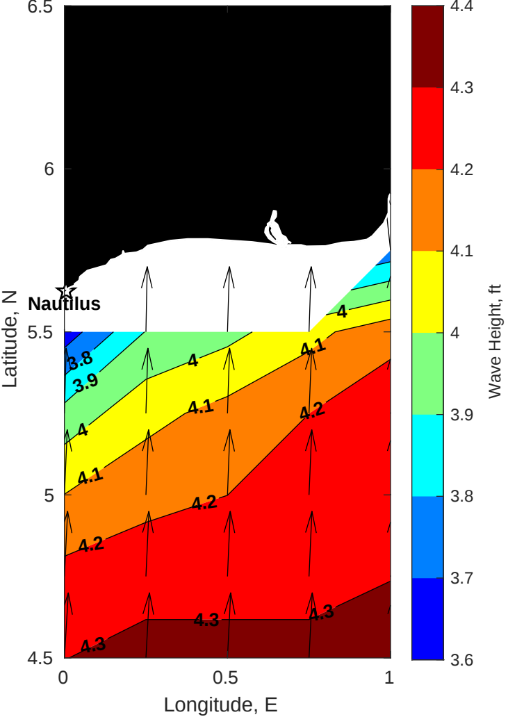
Wave Height (ft) for Nautilus at 13-Sep-2025 09:00:00
