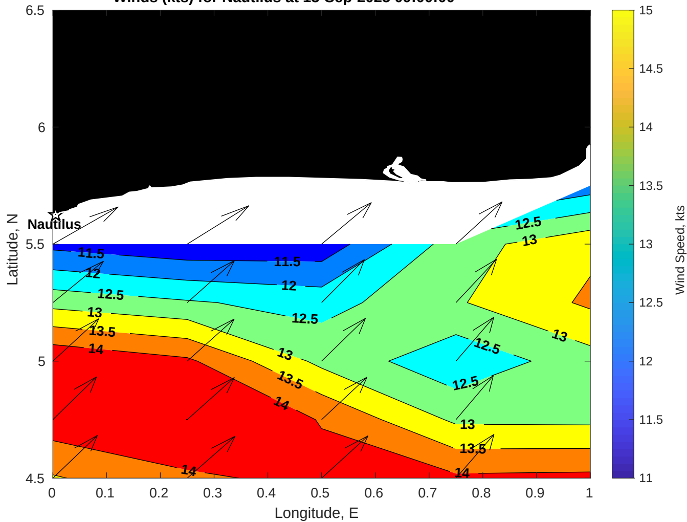
Winds (kts) for Nautilus at 13-Sep-2025 09:00:00
