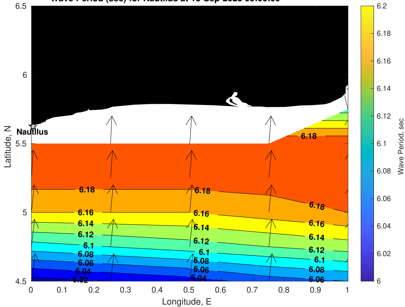
Wave Period (sec) for Nautilus at 13-Sep-2025 09:00:00
