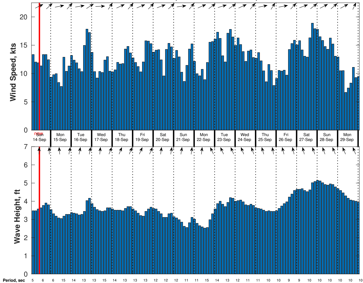
Wind & Wave Forecast for Nautilus from 13-Sep-2025 02:00:00 to 29-Sep-2025 02:00:00
