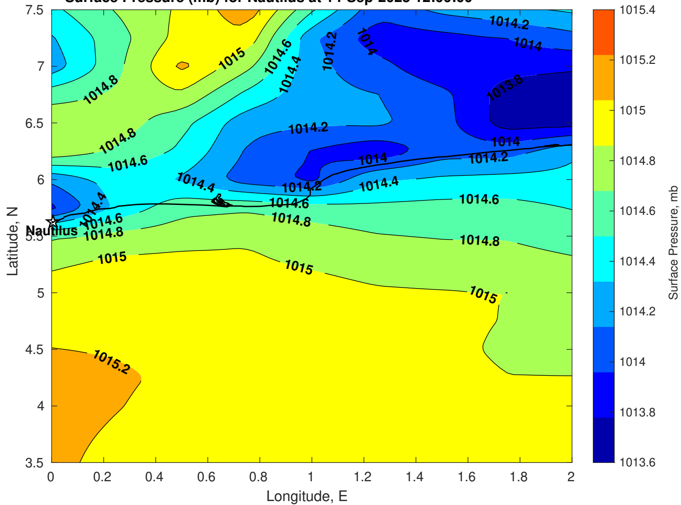
Surface Pressure (mb) for Nautilus at 14-Sep-2025 12:00:00
