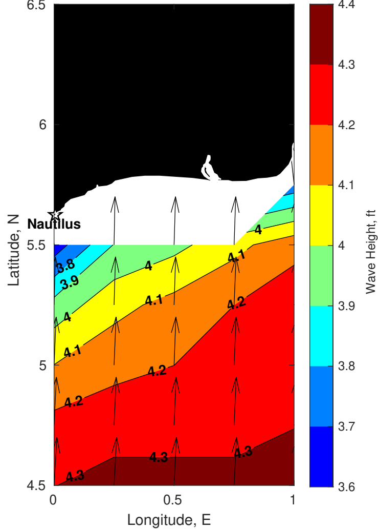
Wave Height (ft) for Nautilus at 13-Sep-2025 09:00:00
