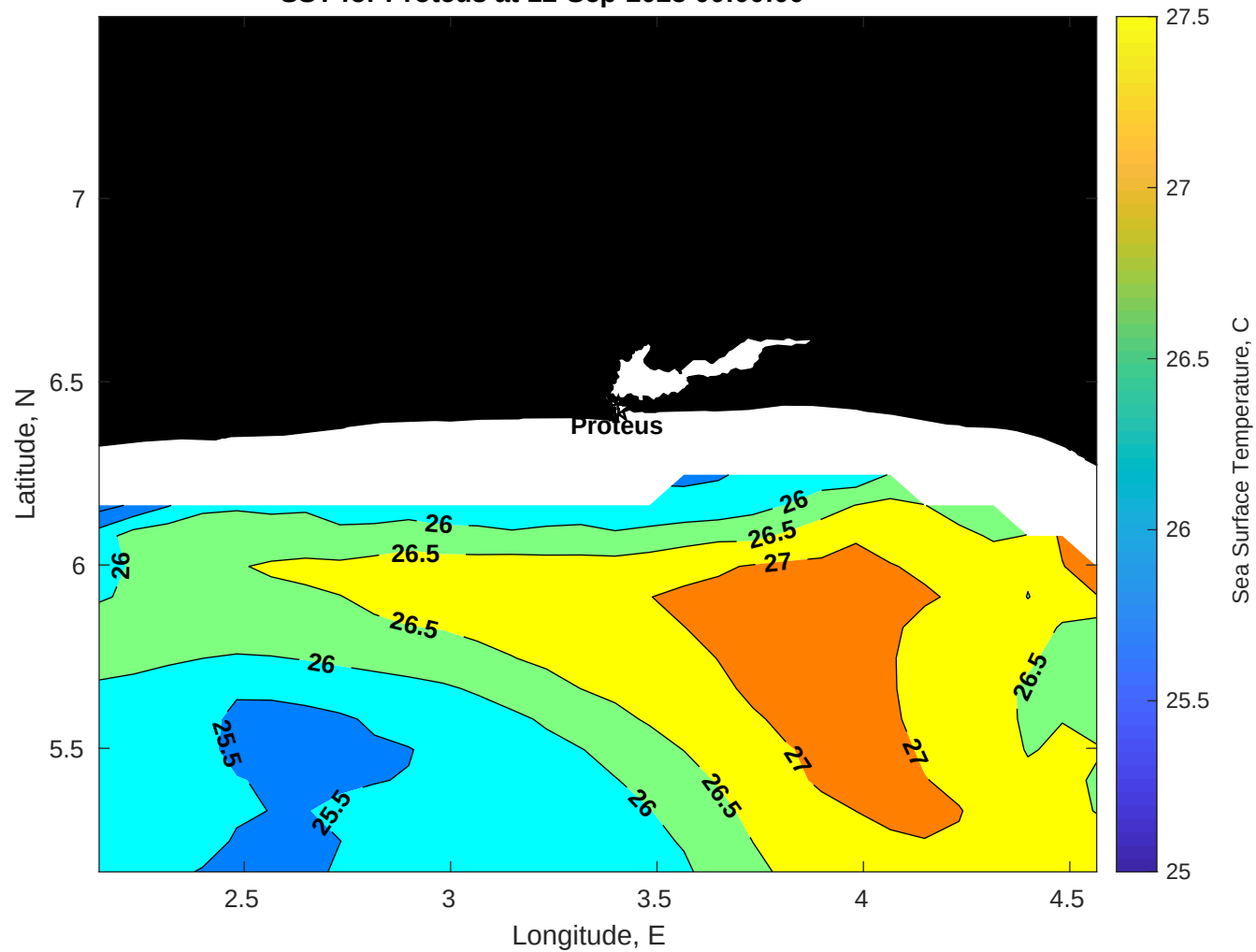
SST for Proteus at 12-Sep-2025 00:00:00
