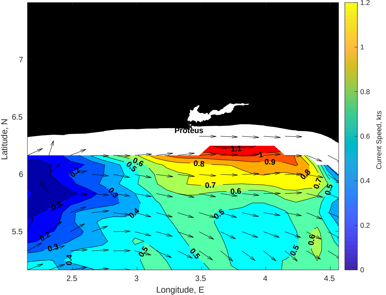
Surface Currents for Proteus at 12-Sep-2025 00:00:00
