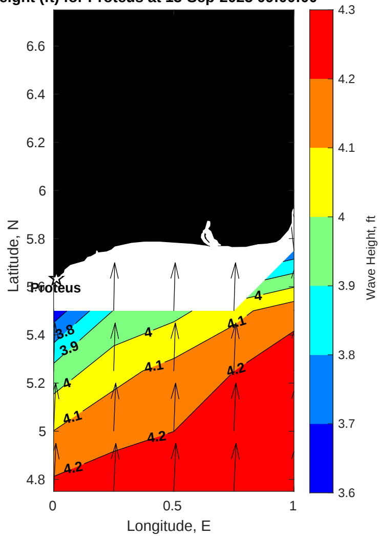
Wave Height (ft) for Proteus at 13-Sep-2025 09:00:00
