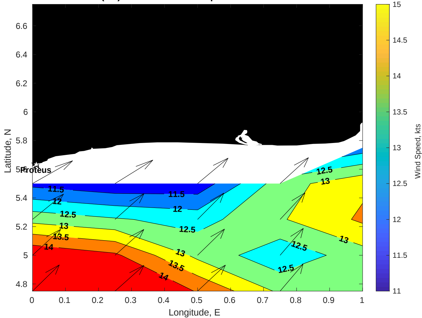
Winds (kts) for Proteus at 13-Sep-2025 09:00:00
