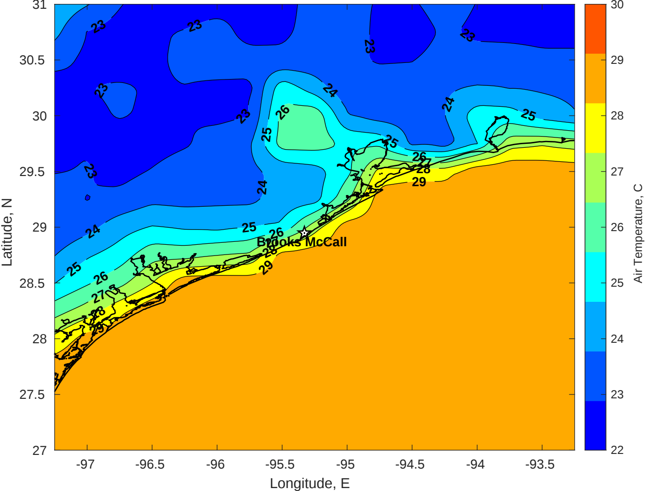
Air Temperature (C) for Brooks McCall at 13-Sep-2025
