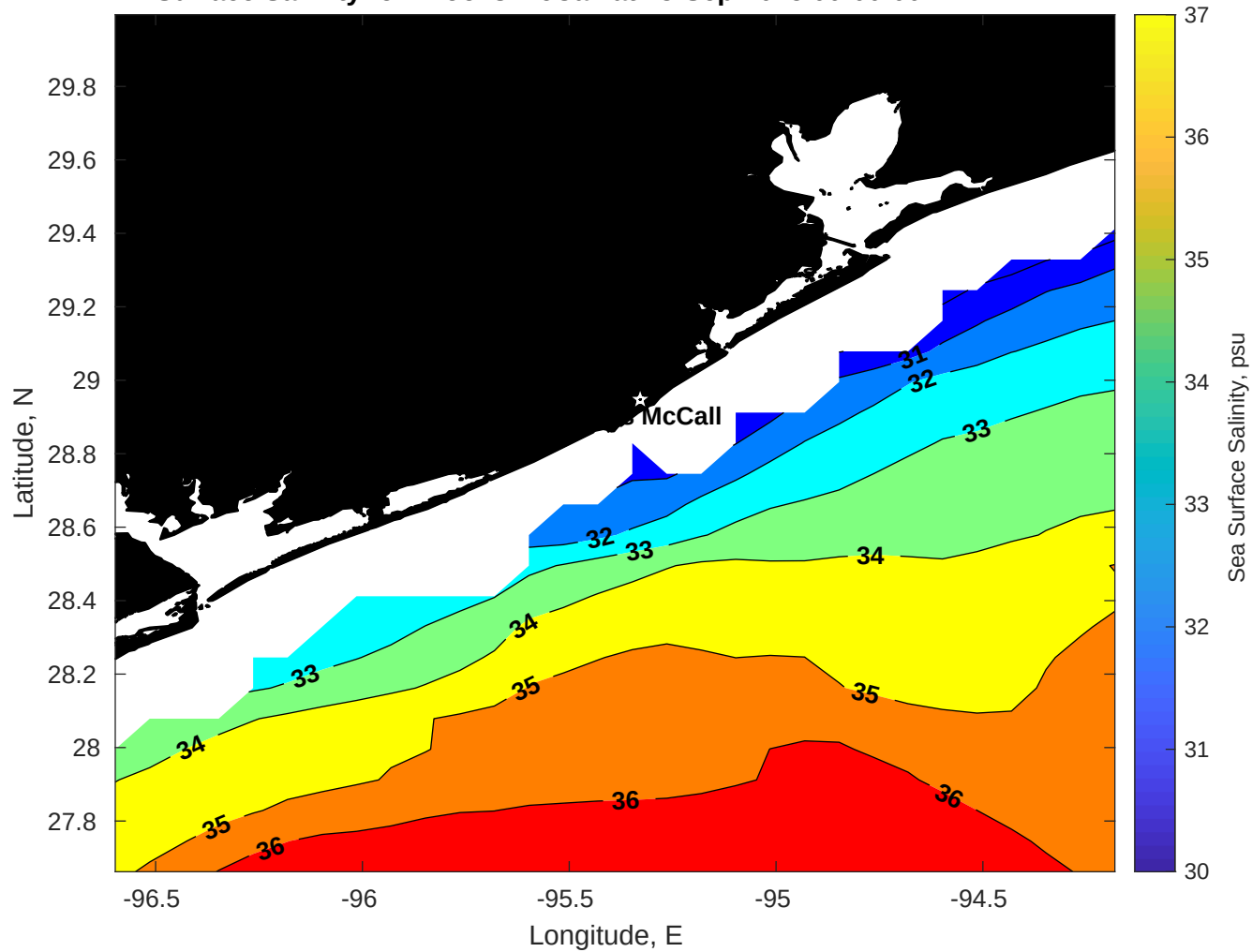
Surface Salinity for Brooks McCall at 13-Sep-2025 00:00:00
