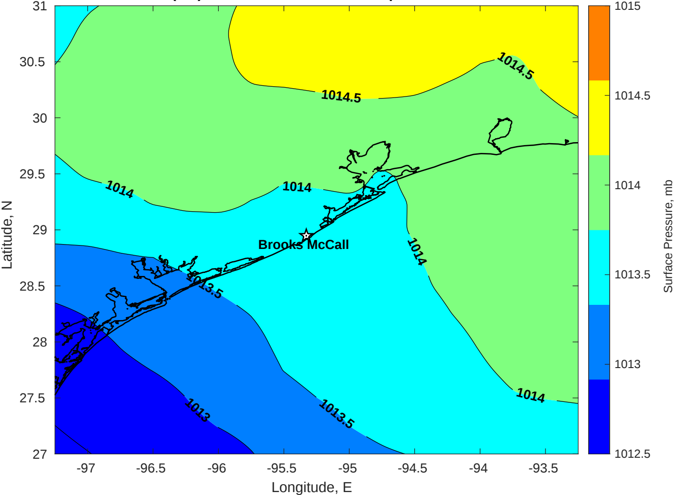
Surface Pressure (mb) for Brooks McCall at 14-Sep-2025 12:00:00
