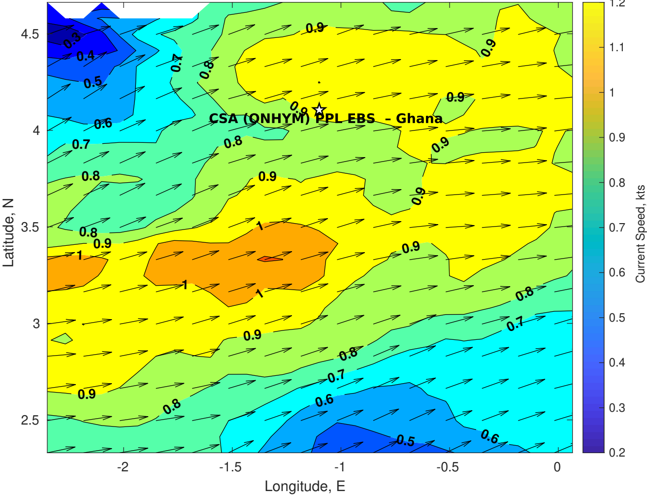
Surface Currents for CSA (ONHYM) PPL EBS - Ghana at 13-Sep-2025 00:00:00
