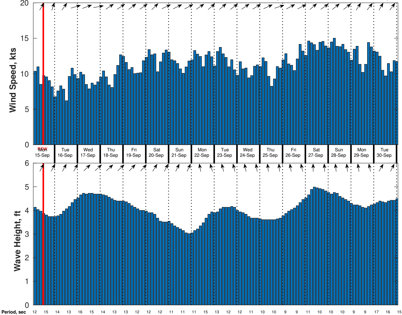
Wind & Wave Forecast for CSA (ONHYM) PPL EBS - Ghana from 14-Sep-2025 02:00:00 to 30-Sep-2025 02:00:00
