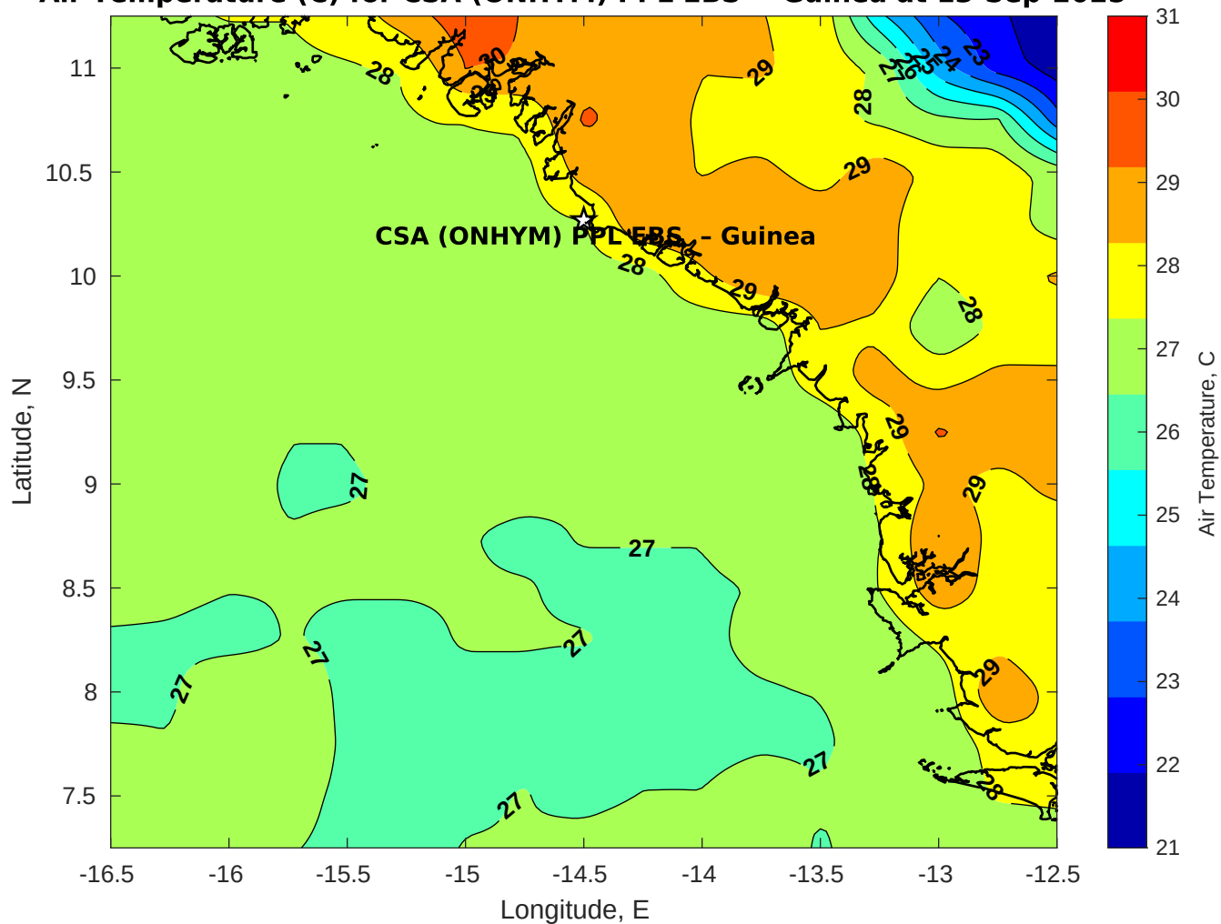
Air Temperature (C) for CSA (ONHYM) PPL EBS - Guinea at 13-Sep-2025
