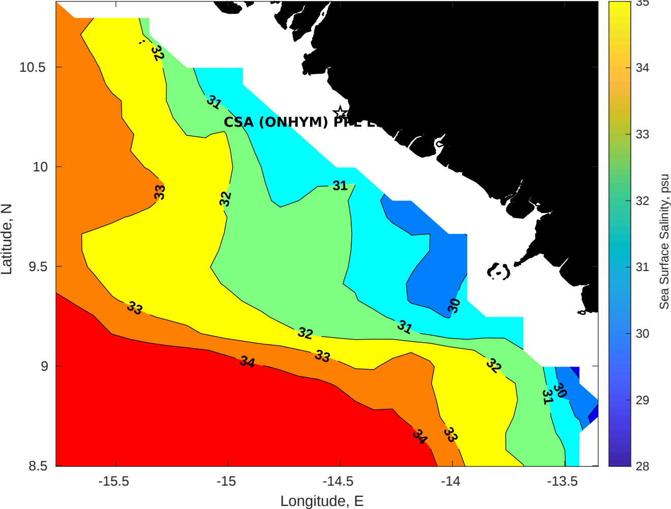
Surface Salinity for CSA (ONHYM) PPL EBS - Guinea at 13-Sep-2025 00:00:00
