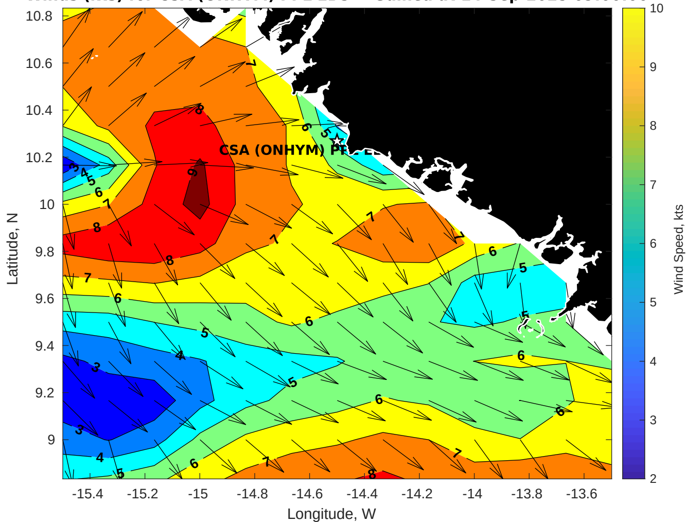
Winds (kts) for CSA (ONHYM) PPL EBS - Guinea at 14-Sep-2025 09:00:00
