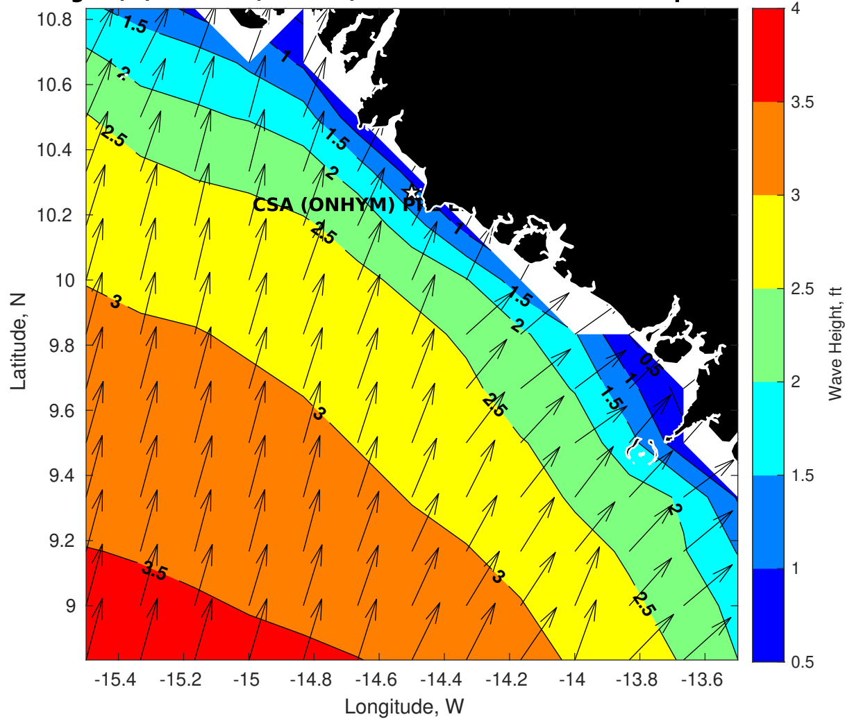
Wave Height (ft) for CSA (ONHYM) PPL EBS - Guinea at 14-Sep-2025 09:00:00
