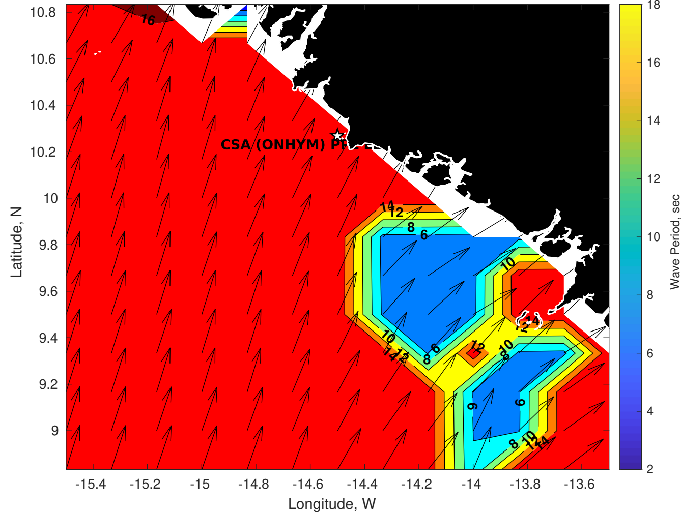
Wave Period (sec) for CSA (ONHYM) PPL EBS - Guinea at 14-Sep-2025 09:00:00
